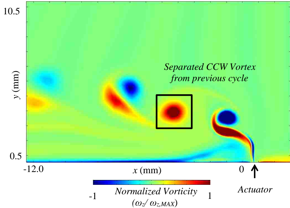
Figure 35 Vorticity contours for single SJA @ t/T = 37.68
