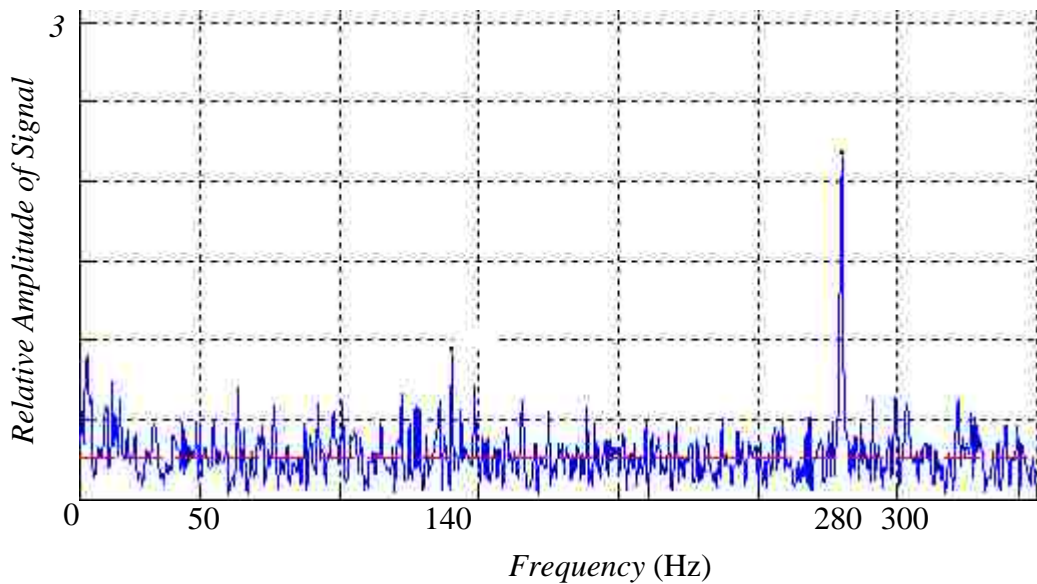
Figure 80 Frequency analysis of PIV data obtained at 8 mm above the orifice (red line indicates average magnitude)
