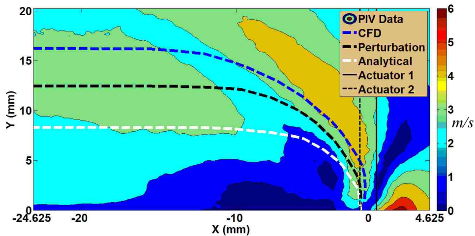
Figure 94 Model validation and flow field analysis for phasing effects \varphi = 60^\circ
