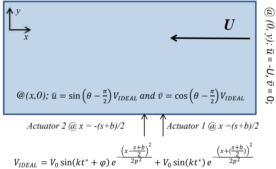
Figure 25 Modified boundary conditions used for analytical modeling
