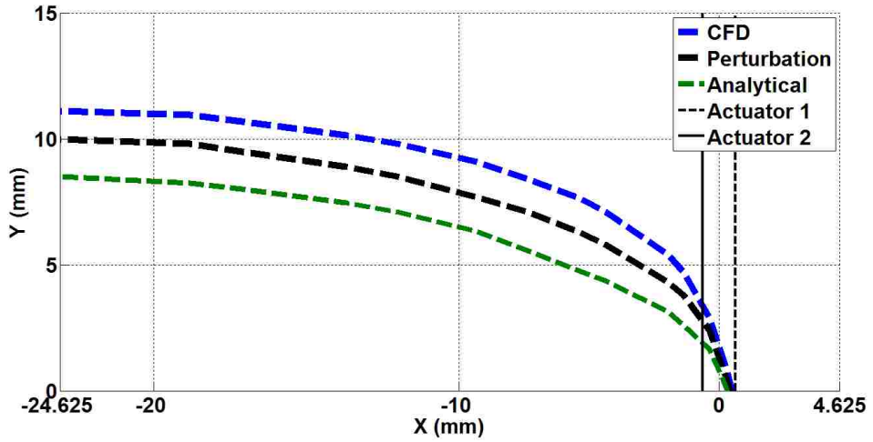
Figure 57 Modeling predictions for jet centerline trajectory for R = 2.4 , s = 2.5b and \varphi = -120^\circ
