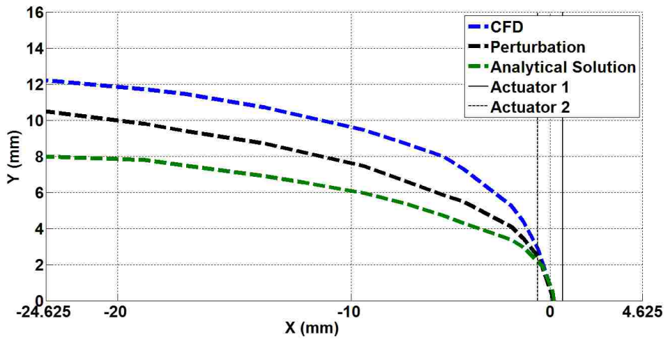
Figure 58 Modeling predictions for jet centerline trajectory for R = 2.4 , s = 2.5b and \varphi = -60^\circ
