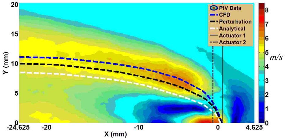
Figure 91 Model validation and flow field analysis for phasing effects \varphi = -120^\circ
