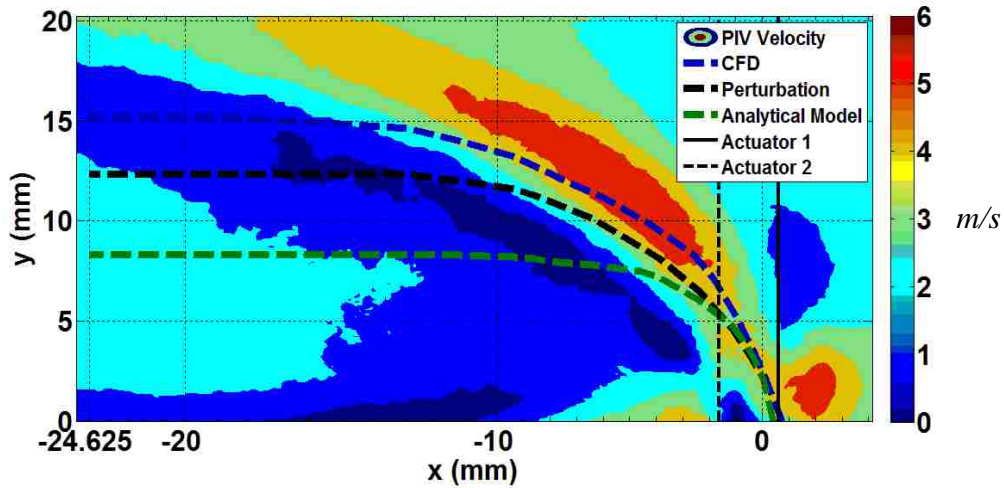
Figure 84 PIV validation of predicted jet centerline trajectories with PIV for R = 2.4 , s = 4.5b , \phi = 0^\circ
