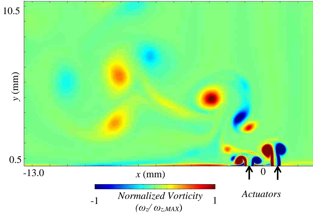
Figure 44 Vorticity contours for dual SJA operating at \phi = 30^\circ @ t/T = 79.22
