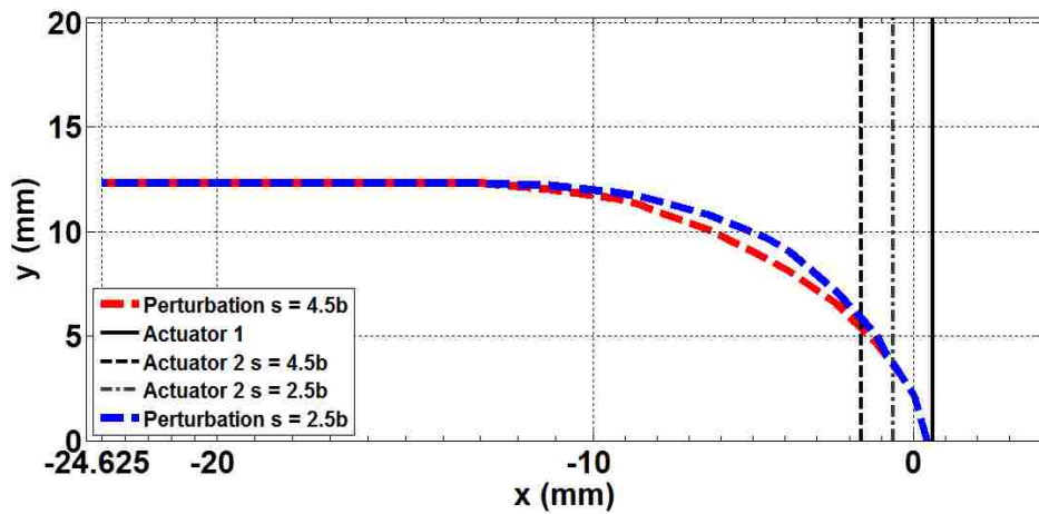
Figure 85 Perturbation predictions for jet centerline trajectory for R = 2.4 , s = 2.5b and 4.5b , \varphi = 0^\circ
