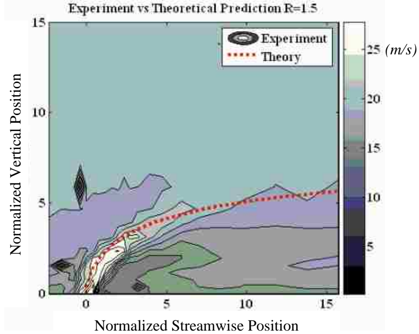
Figure 14 Comparison of jet trajectory analytical prediction with experimental data (Ugrina, 2007)
