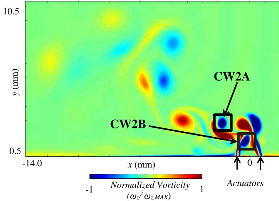
Figure 39 Vorticity contours for dual SJA operating in phase @ t/T = 78.51
