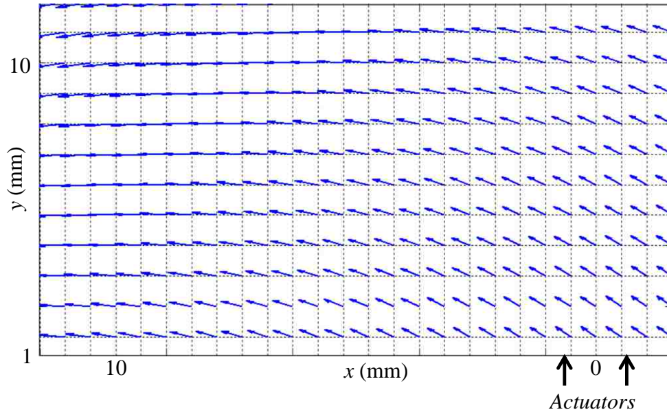
Figure 46 Velocity contours as predicted by analytical solution to perturbation method for dual SJA operating at \phi = 30^\circ @ t/T = 78.30
