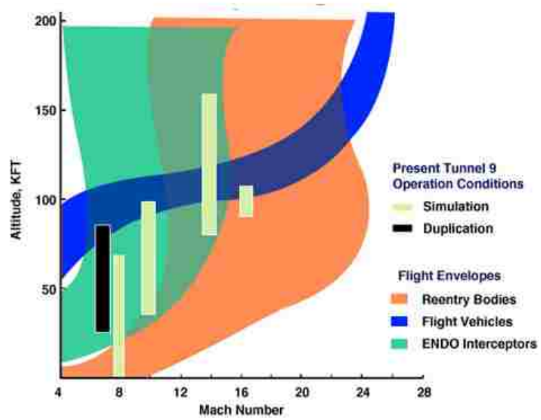
Figure 2.3: Tunnel 9 operational envelope.
