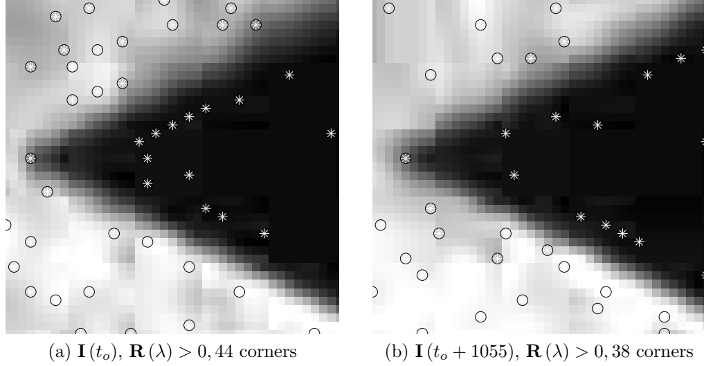
Figure 5.3: Harris corner responses in the model tip ROI shown in \otimes . ROI is 41 x 41 pixels. Responses are spurious, although the cone tip is identified.
