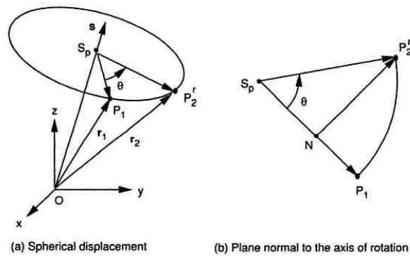
Figure 3.1: Spherical Displacement of A Rigid Body
