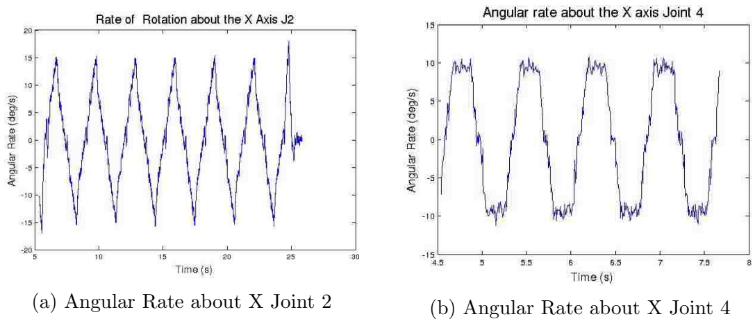
Figure 6.7: Joint Example Angular Rotation
