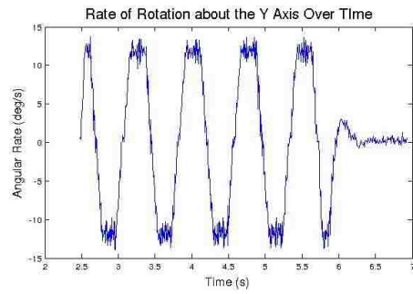
(b) Angular Rate About Y J5
