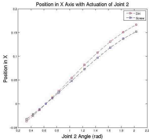
(a) Estimated and Actual X position
