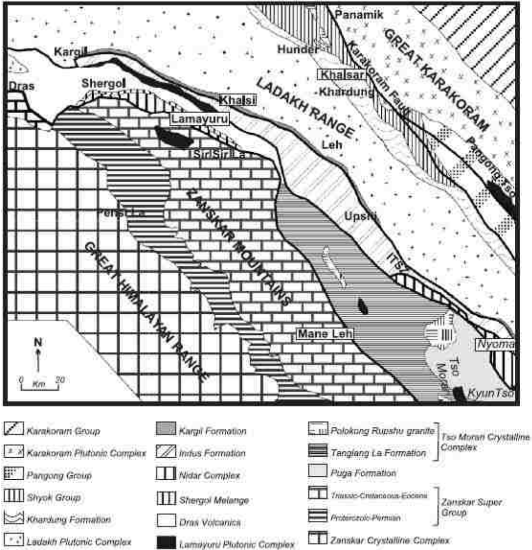
Figure 11. Geological map of Ladakh (Phartiayal et al. 2005).
