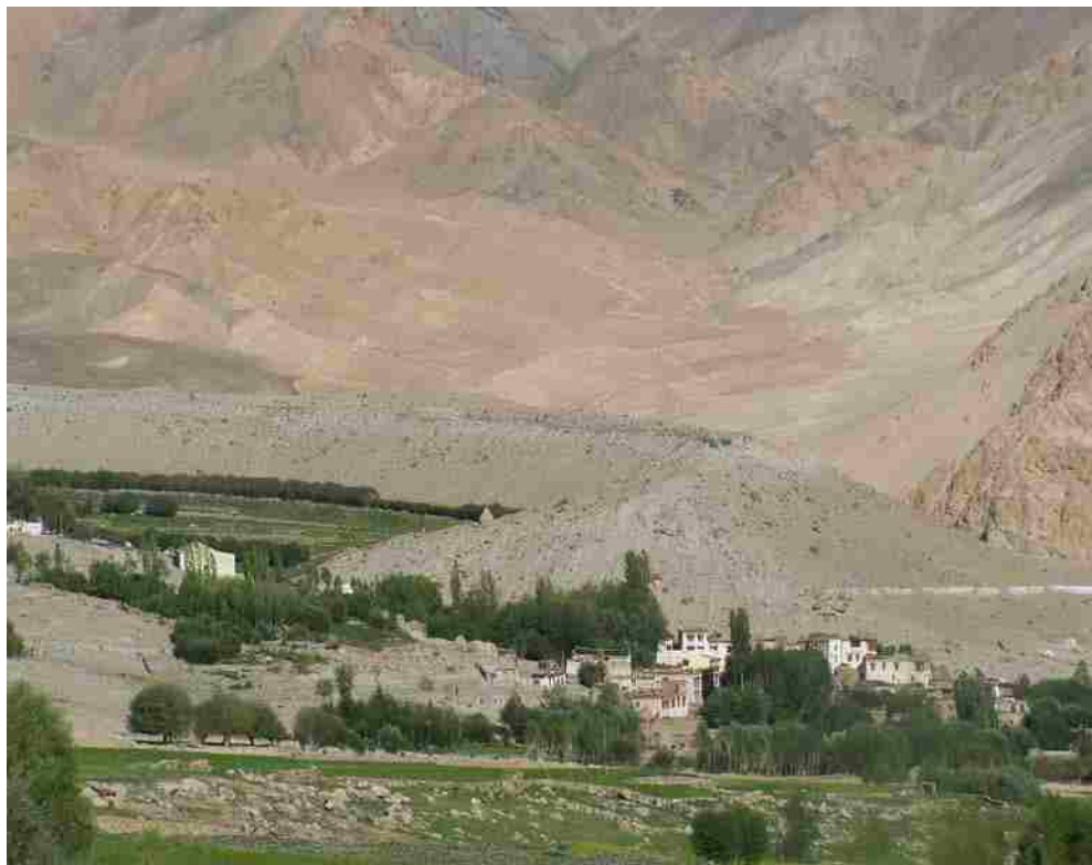
Figure 2. Giant paleomoraine in the Leh Valley, similar to the “huge unfinished railway embankment” described by Lambert (1877). (Photo by M.E. Byrne, 2007).
