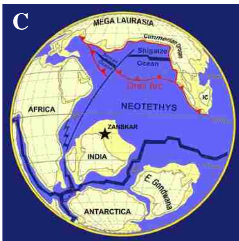
Figure 8. The Indian sub-continent broke away from Gondwana in the Norian, eventually crossing the Neotethys and colliding with Eurasia. (Patriat and Achache 1984; Stampfli and Mosar 1998; Dèzes 1999).
