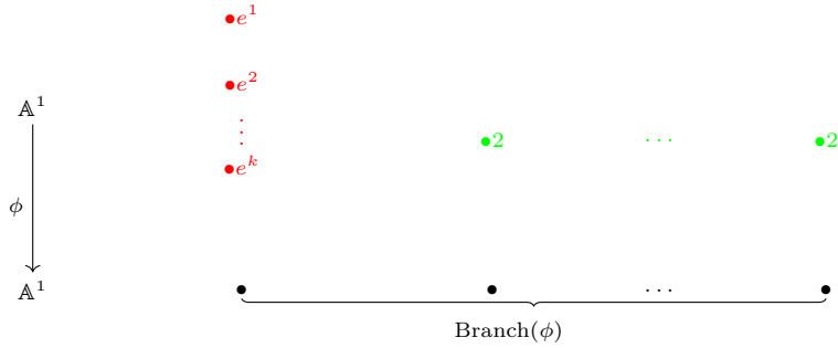
Fig. 6. The above diagram characterizes \lambda \in \mathcal{P}_n such that for any morphism \phi \in \mathcal{I}_\circ \pi(S(\lambda)) , we have that B_b(\phi) = \{2\} for all branch points b \in \text{Branch}(\phi) but one.
