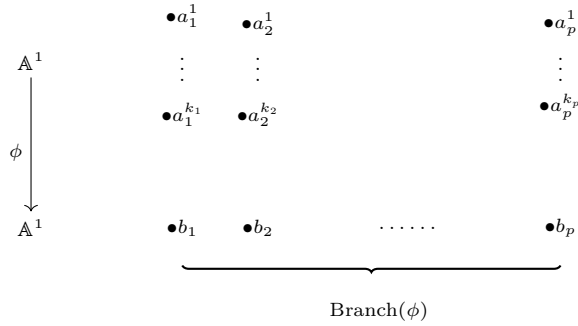
Fig. 2. The diagram above is a schematic of the morphism \phi \in M_n with ramification data given by (2.2).
