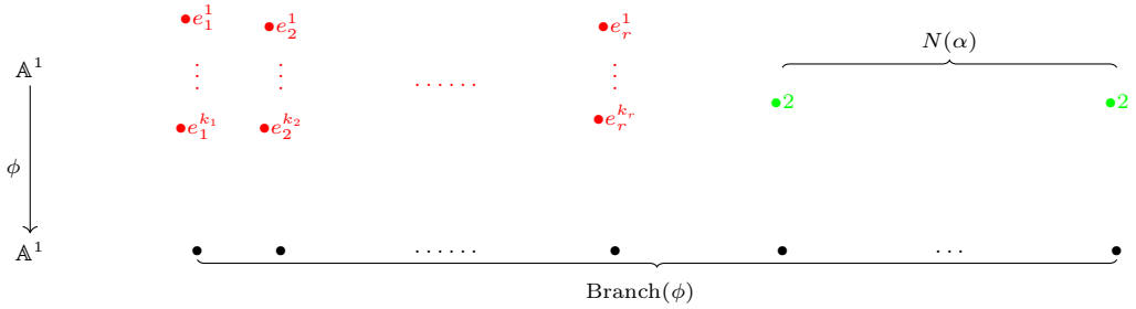
Fig. 4. This is a diagrammatic presentation of the sets N(\alpha), R(\alpha) and F(\alpha) , but only up to permutation by \mathfrak{S}_n . Let \phi \in \mathcal{I}_o\pi(S(\alpha)) . The colored points are the ramification points of \phi , with ramification indices specified. The red points denote the non-simply-branched ramification points of \phi . Counted as per the differential lengths (=ramification index -1 ), they constitute R(\alpha) up to reordering the cells R(\alpha)_i and their elements. The green points, the simply-branched ramification points of \phi , form N(\alpha) . Each “column” of red points (again, counted correctly) is an element in F(\alpha) . (For interpretation of the colors in the figure(s), the reader is referred to the web version of this article.)
