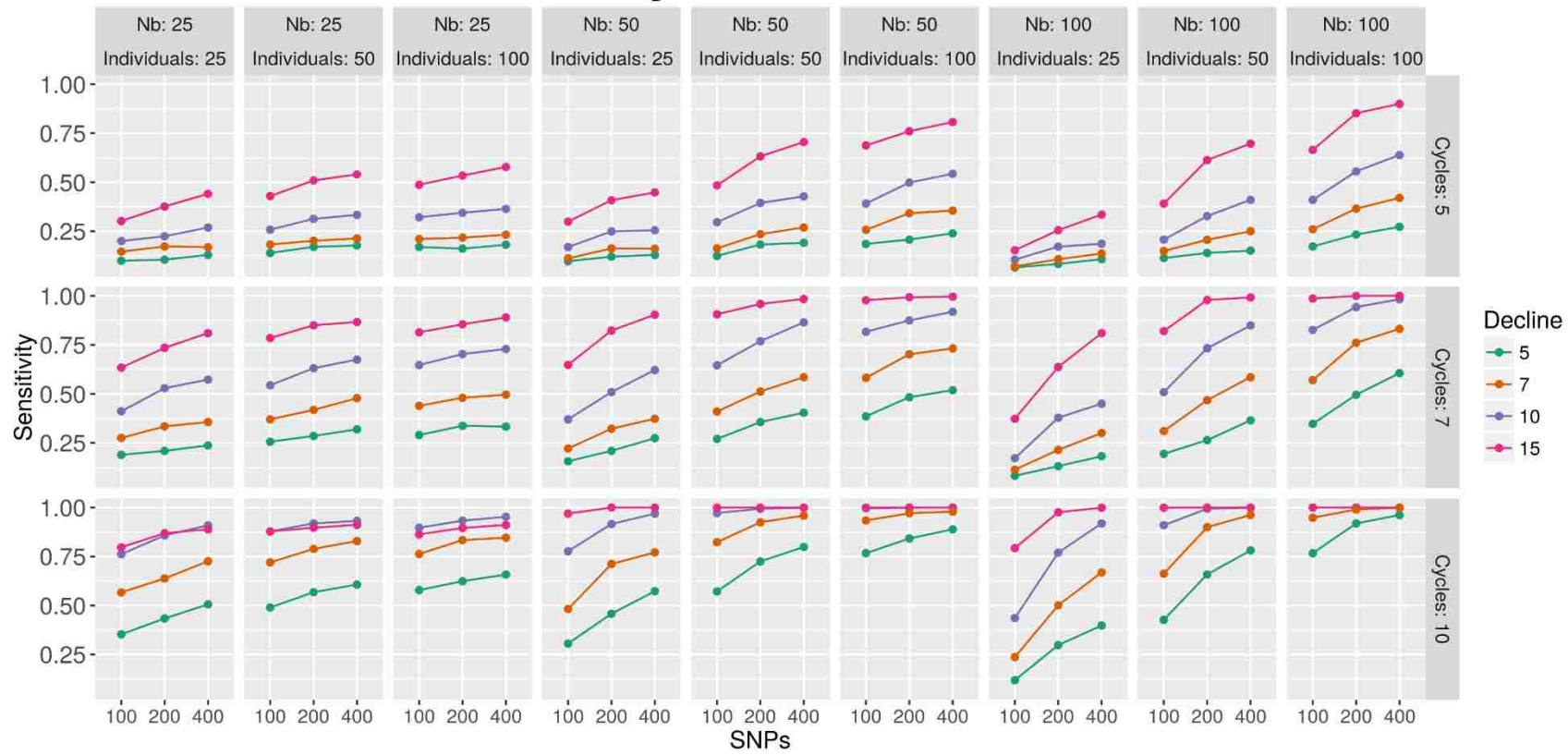
Figure 7: Sensitivities by decline for wood frog at 90% p-value
