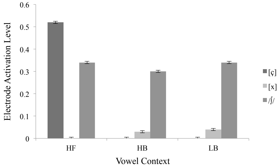
Figure 3. Level of activation and standard error of the mean for [ç], [x], and /j/ given a high-front (HF), a high-back (HB), or a low-back (LB) vowel context and collapsed across word type (real/nonsense), participant, region, and right/left side.
