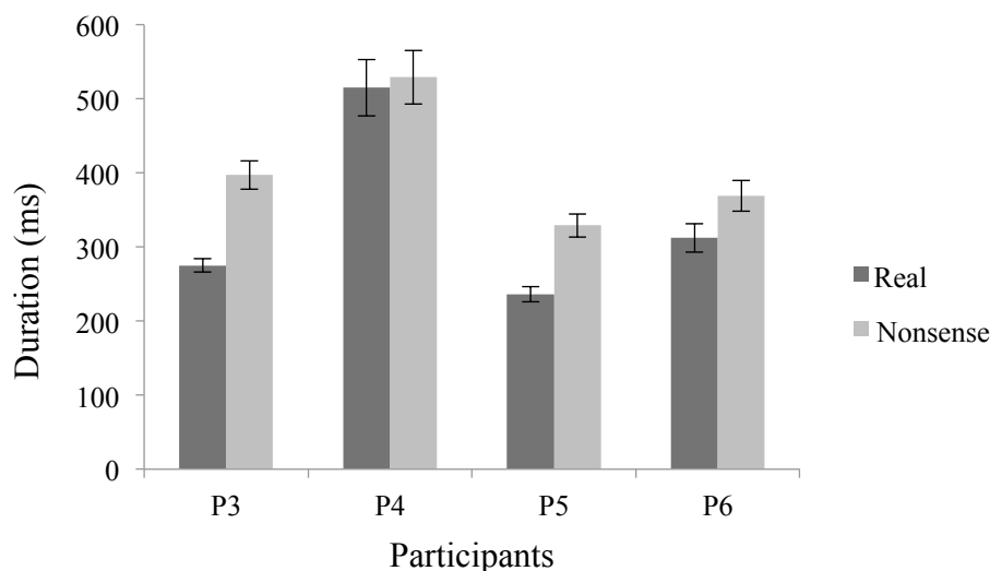
Figure 2. Mean fricative duration and standard error of the mean for real and nonsense words in milliseconds (ms) collapsed across all sounds and vowel contexts for each participant (P).
