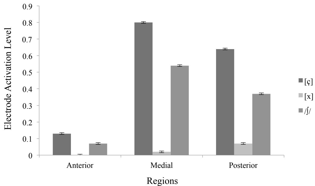
Figure 4. Electrode activation level within each region, collapsed across right/left side, word type (real/nonsense), participant, and vowel context.
