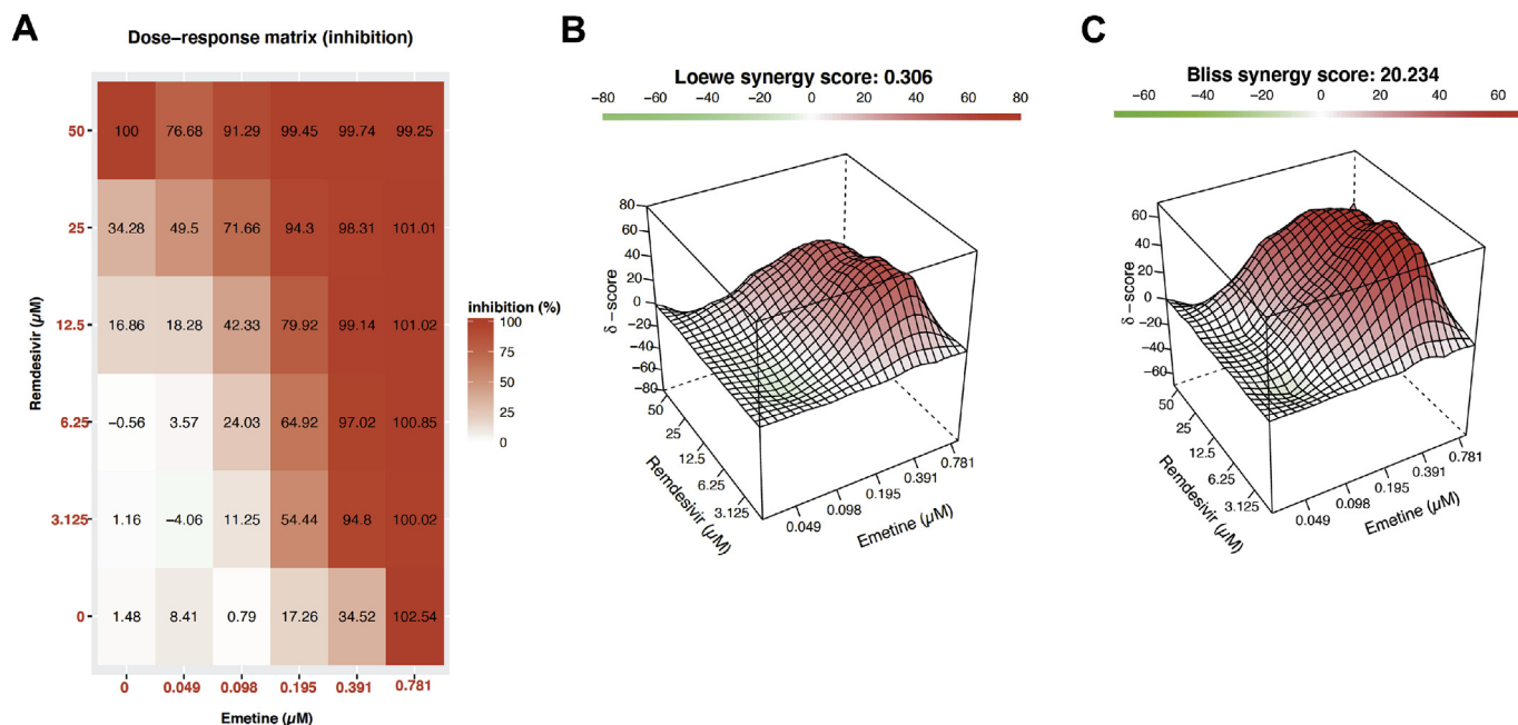
Fig. 2. Combinational effect of remdesivir and emetine dihydrochloride against SARS-CoV-2 virus in vitro. (A) Dose response matrix of serially 2-fold diluted remdesivir (0–50 μM) and emetine (0–0.781 μM) in Vero E6 cells. The percentage of viral inhibition was normalized based on viral load in logarithm scale ( \log_{10}RNA copies/mL), using the maximal viral RNA copies with no drug controls as 0% inhibition and the minimal RNA copies determined at 50 μM remdesivir as references. (B) The three-dimensional interaction landscapes of remdesivir and emetine were generated by SynergyFinder (Ianevski et al., 2017) based on (B) the Loewe additive model and (C) the Bliss independence model. Red colour indicates synergy while the green colour indicates antagonism of the two drugs.
