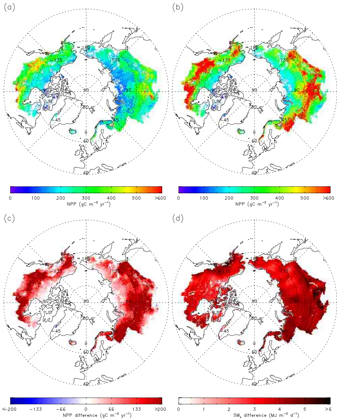
Figure 2-6: Mean annual NPP ( \text{g C m}^{-2} \text{ yr}^{-1} ) derived from PEM calculations driven by ERA-40 (a) and NNR (b) over the pan-Arctic domain and 19-year (1982-2000) study period. The NPP (c) and SW_1 (d) difference maps refer to NNR less ERA-40 results.
