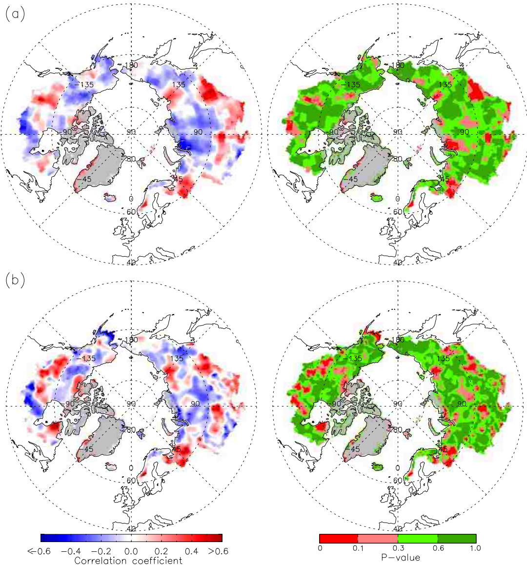
Figure 5-7: Maps of correlations between PDO_{GS} and GS P-ET and corresponding P -values; the top graphs are derived using GPCP precipitation while the bottom graphs are derived using GPCP precipitation.
