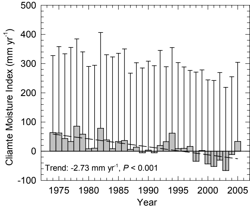
Figure 3-17: Mean annual climate moisture index ( P-PET ) for the pan-Arctic basin and Alaska domain and 1974–2005 period; error bars denote the standard deviation of annual observations for the domain. The total number of NCDC CSB stations used to compute the index ranged from 2053 to 2924 per year.
