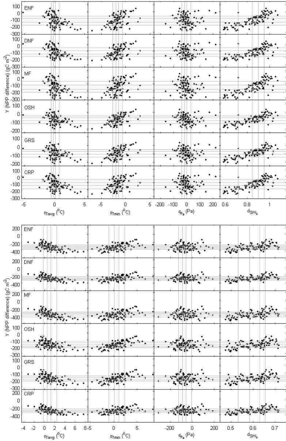
Figure 2-5: Scatter plots of Y vs. \epsilon_{Tavg} , \epsilon_{Tmin} , \epsilon_{ea} and d_{SW1} from ERA-40 (top) and NNR (bottom) for the six general biome types. The 5 \times 5 grid for the SI and entropy tests is also shown in the graphs.
