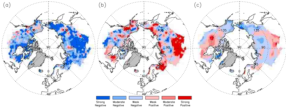
Figure 3-9: Spatial patterns of changes in growing season (GS, April to October) (a) I_t , (b) I_m , and (c) SW_l across the pan-Arctic region from 1983 to 2005.
