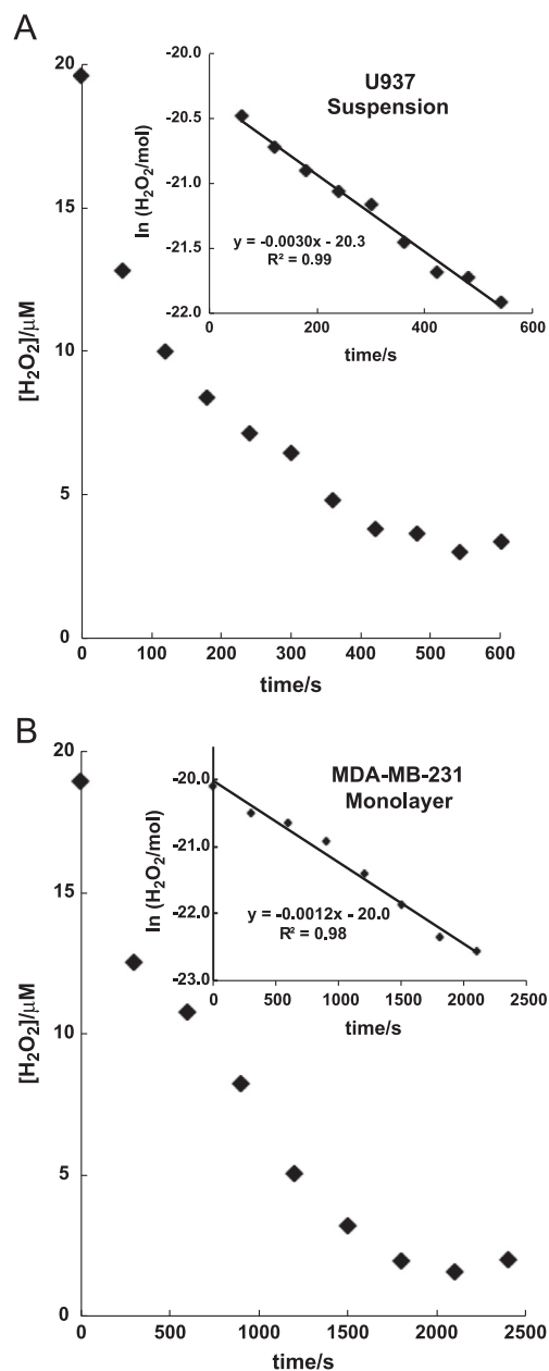
Fig. 3. Removal of extracellular H 2 O 2 by cells grown in suspension culture or as adherent monolayers is a first-order process. (A) U937 cells ( 5.0 \times 10^4 cells well -1 ) in HBSS were incubated with 20 μM H 2 O 2 for 0–10 min (100 μL total volume) at room temperature and then assayed for the remaining extracellular H 2 O 2 using the pHPA assay. The observed first-order rate constant for the loss of extracellular H 2 O 2 in this experiment was determined to be k_{\text{obs}} = 3.0 \times 10^{-3} \text{ s}^{-1} . The cell density in this experiment was 5.0 \times 10^8 cells L -1 . This yields k_{\text{cell}} = k_{\text{obs}} / (5.0 \times 10^8 \text{ cell L}^{-1}) = 6.0 \times 10^{-12} \text{ s}^{-1} \text{ cell}^{-1} \text{ L} . (B) MDA-MB-231 human breast cancer cells ( 2.1 \times 10^5 cells well -1 ) were allowed to attach overnight to the bottom of the tissue culture well, rinsed of old media, and washed with HBSS and covered with 50 μL HBSS. The cells were then treated with 20 μM H 2 O 2 (100 μL total volume); because of their much lower capacity to remove extracellular H 2 O 2 the time of maximum exposure was 40 min. The observed first-order rate constant for the loss of extracellular H 2 O 2 in this experiment was determined to be k_{\text{obs}} = 1.2 \times 10^{-3} \text{ s}^{-1} . The cell density in this experiment was 2.1 \times 10^9 cells L -1 . This yields k_{\text{cell}} = k_{\text{obs}} / (2.1 \times 10^9 \text{ cell L}^{-1}) = 0.57 \times 10^{-12} \text{ s}^{-1} \text{ cell}^{-1} \text{ L} . Both experiments are representatives of typical observations seen in greater than 50 experiments with various cell lines.
