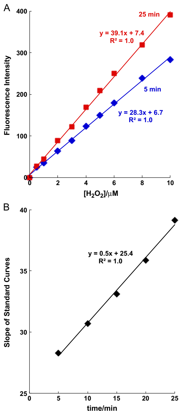
Fig. 2. A typical standard curve performed under the conditions of the assay for removal of extracellular H 2 O 2 by cells. (A) Representative standard curve from a HRP/pHPA-based assay for H 2 O 2 read with a fluorescence plate reader. The data are the average of triplicate samples on a plate read 5 and 25 min after addition of the stopping solution. The lower limit of detection (LLD) for the 25-min standard curve was 0.43 μM. (B) The slope of a standard curve changes linearly with time. Here the plate with the standard samples was read at five different times (5–25 min) after addition of the stopping solution. Again, this demonstrates that standards and samples must be run in parallel with steps in the protocol being congruent as appropriate.
