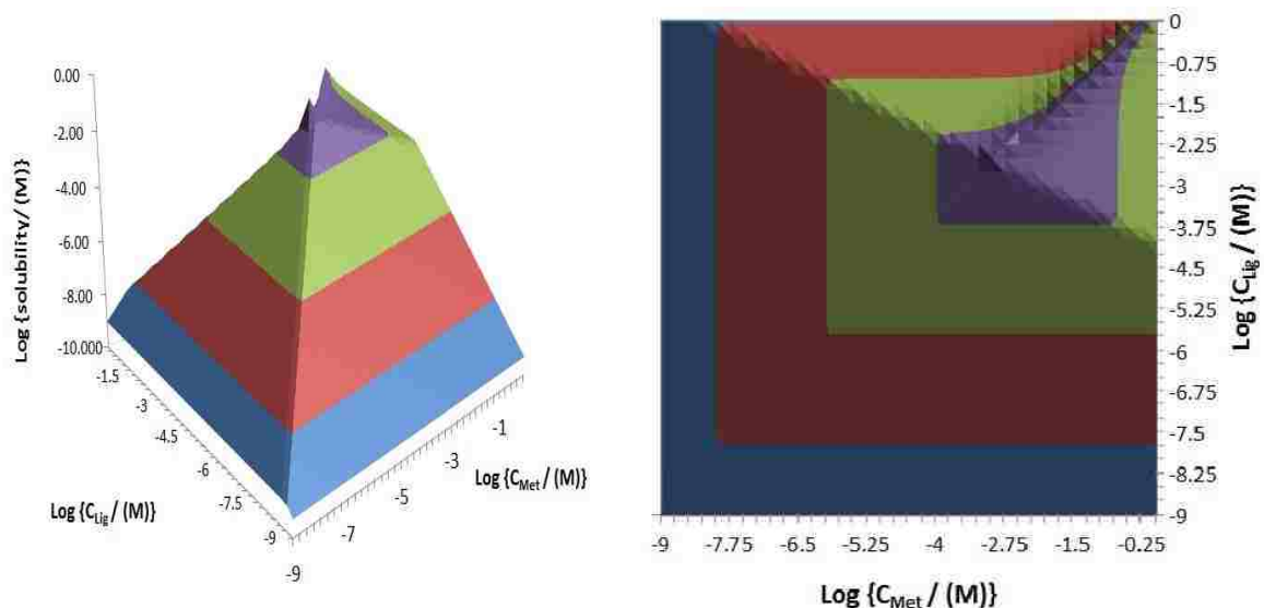
Figure 8.4. Colored wire frame and contour map solubility topos for \text{PbI}_2
