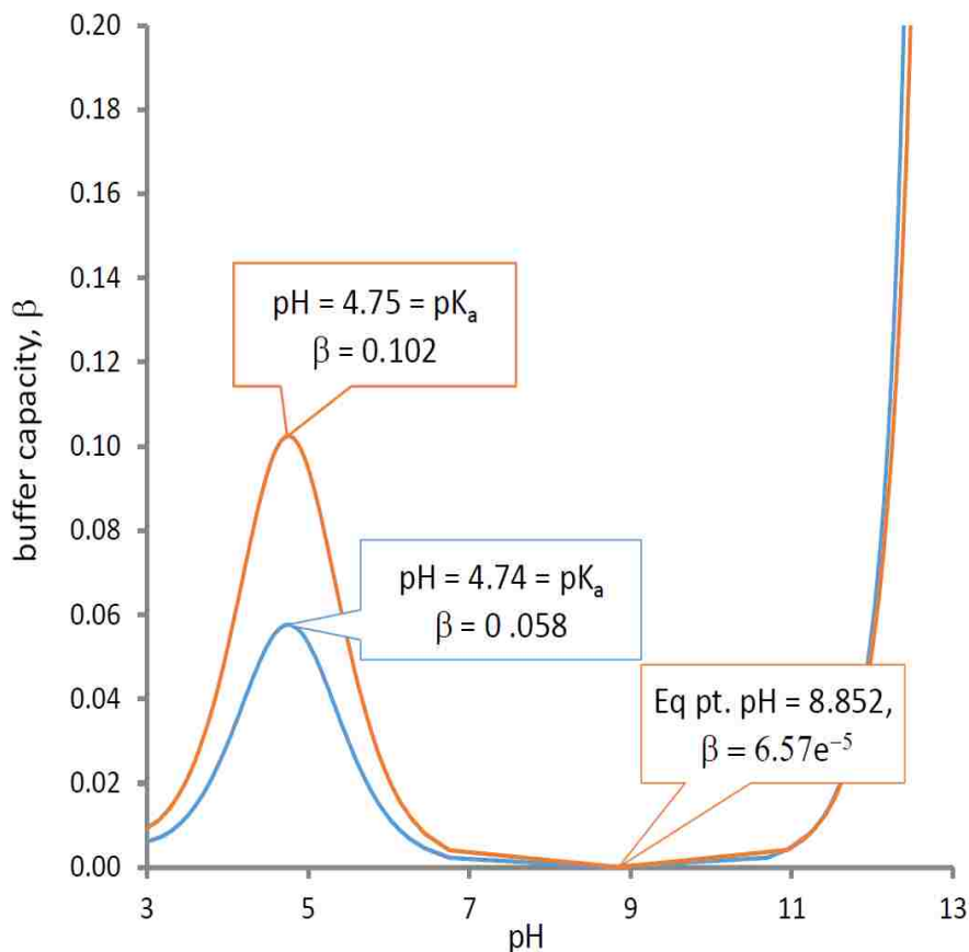
Figure 4.2. Buffer capacity vs. pH for acetic acid ( \text{pK}_a = 4.75 ) at 0.1000 M and 0.1778 M concentrations.
