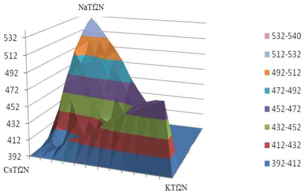
Figure 2.4. 3-Dimensional wire-frame compositional representation of Figure 2.3.
