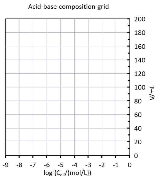
Figure 2.8. The typical composition grid for acid-base titration dilution topo surfaces. For simpler representation number of grid points are reduced. The orientation of the composition grid is rotated 90° counter-clockwise to match the viewing angle of the topos presented in Chapters 3 and 4.
