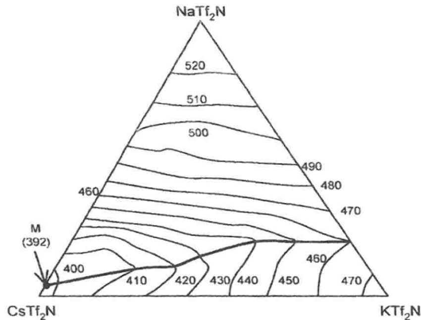
Figure 2.3. Compositional changes in a ternary system with temperature. Molten electrolyte compositions vary in their sodium, cesium and potassium triflet contents as a function of temperature 18 .
