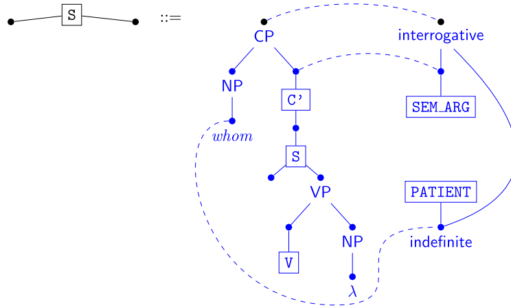
Fig. 13. Lexicon entry for fronted wh -phrases. The nonterminal labelled v is the predicted thematic role assigner.
