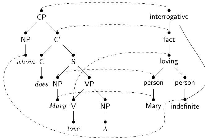
Fig. 19. Millstream configuration for the question Whom does Mary love?
