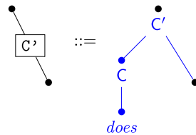
Fig. 14. Lexicon entry for does as an auxiliary in a question.
