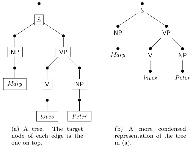
Fig. 2. Pictorial representation of a term graph without sharing, that is, a tree.
