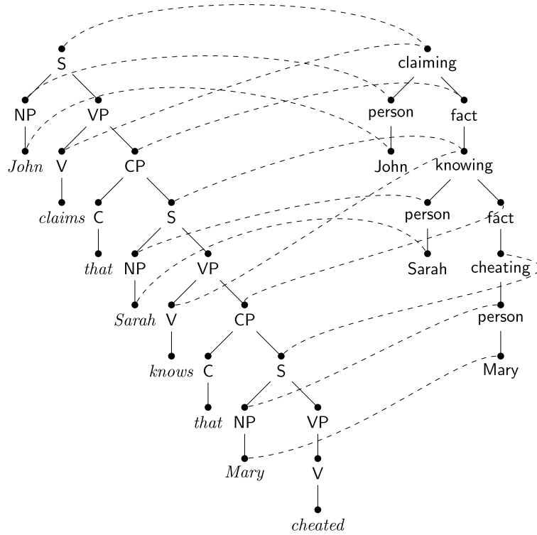
Fig. 12. Millstream configuration including the syntactic and semantic structures of the sentence John claims that Sarah knows that Mary cheated .
