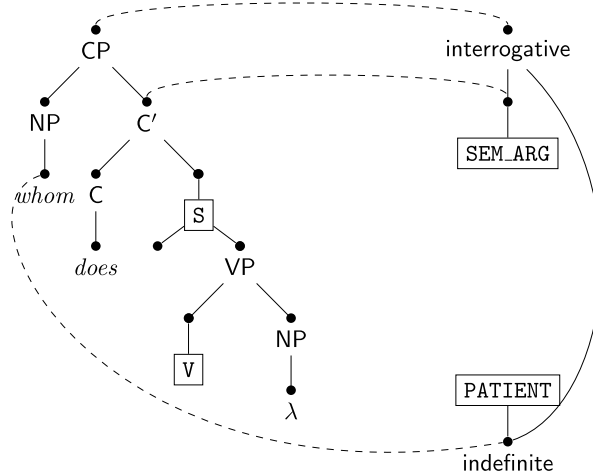
Fig. 17. Partial Millstream configuration for whom does . The syntactic thematic role assigner and the thematic role of the indefinite entity, indicated by the nonterminals labelled V and PATIENT , respectively, need to be specified during further reading.
