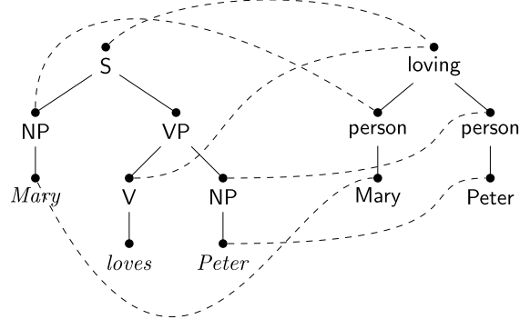
Fig. 3. A sample configuration that relates a syntactic and a semantic tree.
