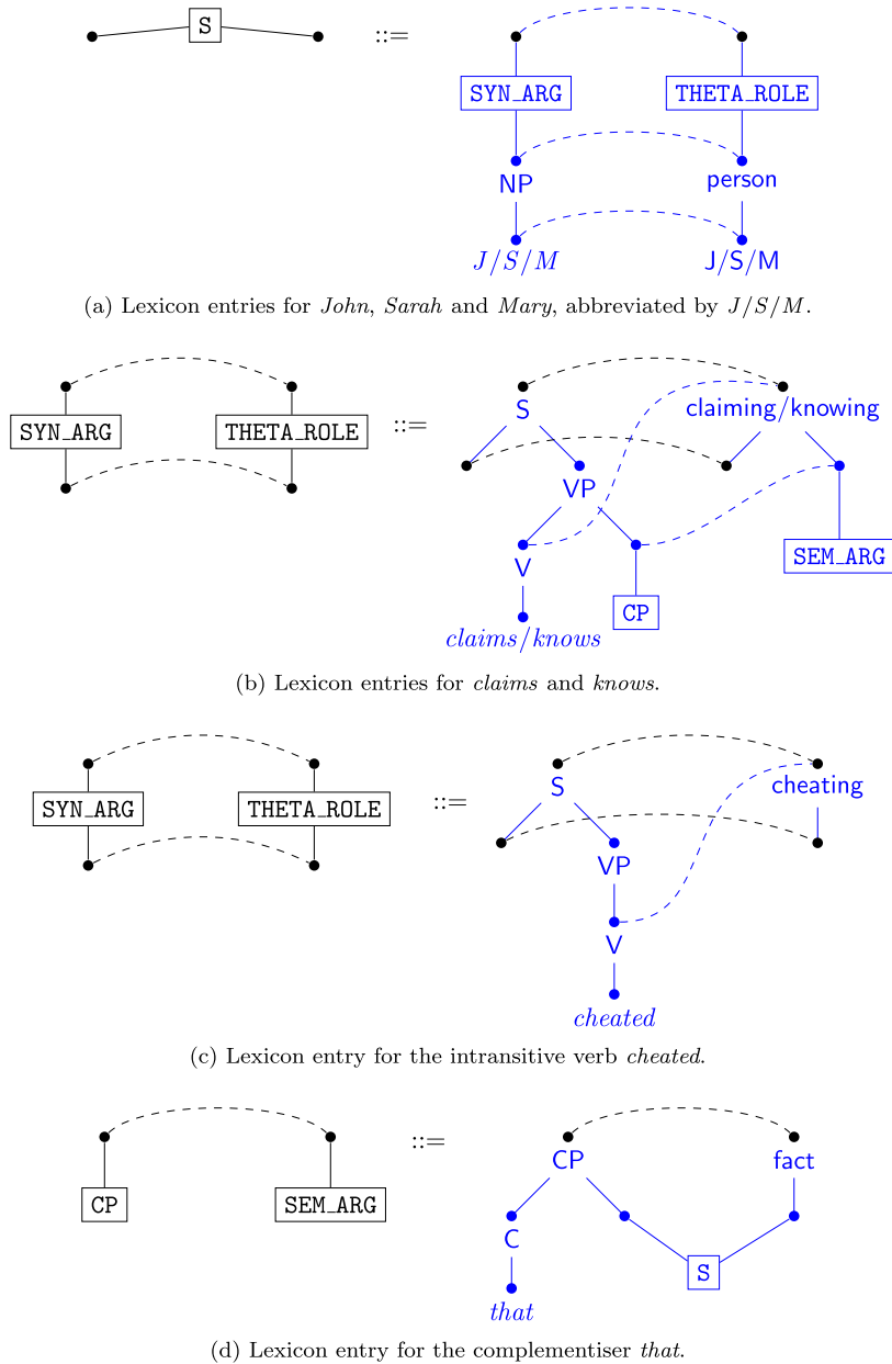
Fig. 11. Handling embedding in John claims that Sarah knows that Mary cheated.
