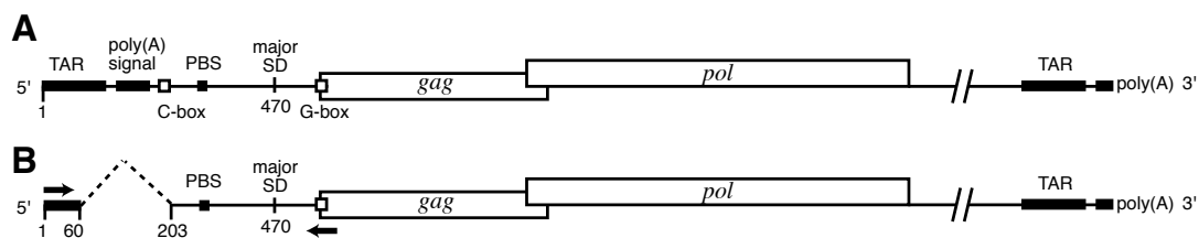
Figure 10. Schematic of the two forms of HIV-2 gag (and gag-pol) mRNAs. The two forms are 5'UTR-unspliced (A) and 5'UTR-spliced (B), respectively. TAR, poly(A) signal, C-box, PBS, major SD, G-box, gag, and pol represent the transactivation region, the poly(A) signal domain, the core of the C-box, the tRNA primer binding site, the major SD site, the core of the G-box, the Gag protein coding region, and the Pol protein coding region, respectively.
