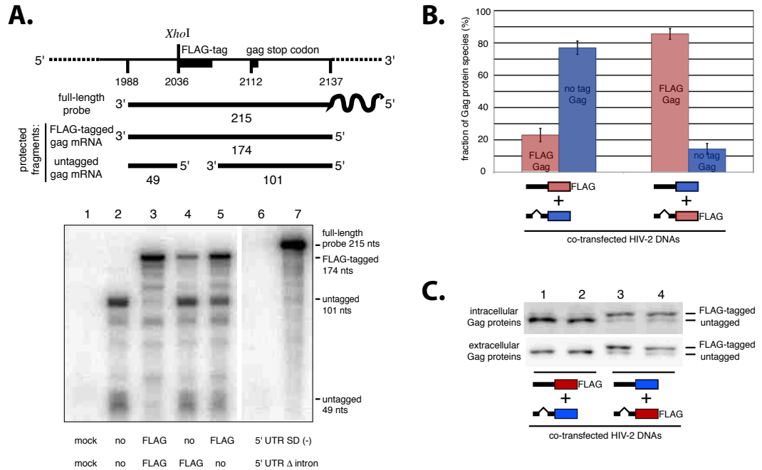
Figure 14. Effects of the 5'UTR intron on HIV-2 gag mRNA and protein species in cell culture. (A) (Top) Schematic of the radioactively labeled probe and predicted protected fragments based on the presence or absence of the FLAG tag. (Bottom) Rnase protection assay of intracellular RNAs. Lane 1 contains the mock-transfected sample. DNA templates used for each cotransfection are designated below each respective lane (lanes 2-5). Lanes 6 and 7 represent yeast RNA used as a nonspecific target RNA control, incubated with and without Rnases, respectively. (B) Quantitation of Gag protein species produced in the cytoplasm of cells cotransfected with 5'UTR SD(-) and Δ-intron HIV-2 plasmid DNA, with the FLAG-tag inserted in one or the other plasmid. The levels of the Gag protein species produced, either FLAG-tagged or untagged, were quantified from a Western blot assay (Figure 13C, lanes 4 and 5) and then corrected for the level of their corresponding mRNA (A, lanes 4 and 5). Three experiments were used to determine the fraction of Gag protein species in each cotransfection. A schematic of the cotransfected plasmid DNAs used is shown below the graph. (C) Western blots of intracellular and extracellular (virion fraction centrifuged from cell culture media) Gag protein. A schematic of the cotransfected plasmid DNAs used is shown below the blots. The blots show both the intracellular and extracellular fractions contain a majority of Gag derived from the Δ-intron construct, and that both the FLAG-tagged and untagged Gag are present without discrimination in the virus fraction.
