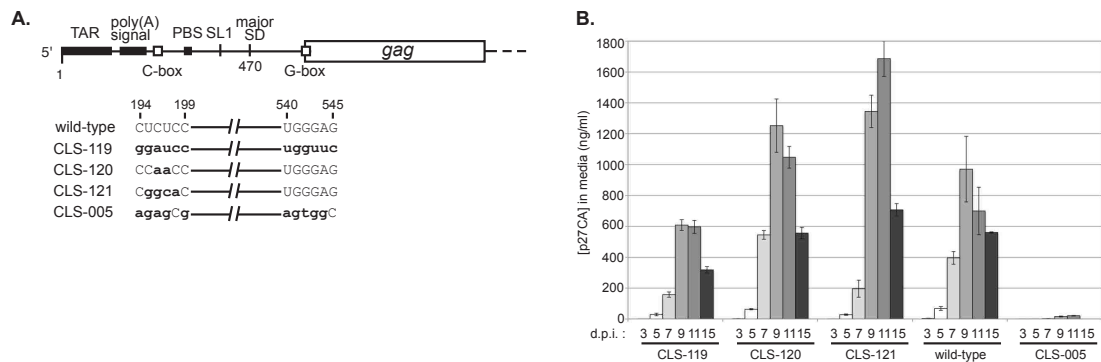
Figure 25. Replication kinetics of mutant HIV-2 viruses.
