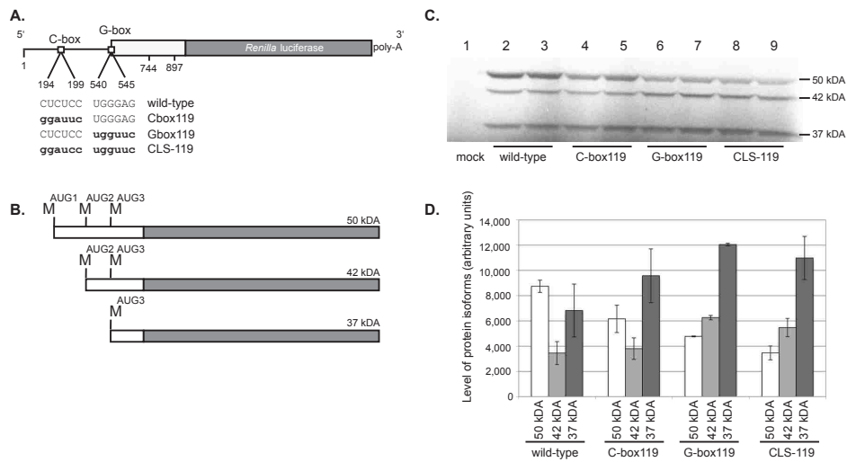
Figure 31. In vitro translation of luciferase mRNAs harboring mutated HIV-2 5' leaders. (A) A schematic of the four mRNA constructs used in S^{35} in vitro translation assays. The mutated nucleotides are in bold lowercase letters. (B) A schematic of the three HIV-2 Gag-luciferase fusion protein isoforms that are synthesized in vitro . The 50, 42, and 37 kDa isoforms are synthesized when translation initiates from methionine codons located at positions 546, 744, and 897, respectively. (C) Duplicate S^{35} in vitro translation assays of the wild type, C-box119, G-box119, and CLS-119 mRNAs. Lane 1 contains a mock where no mRNA was added to the translation reaction. RNAs used in each translation reaction are indicated below each lane. (D) Quantification of protein isoform expression levels. The RNAs used are indicated on the x-axis, along with the protein isoforms produced and quantified. The level of protein isoforms in arbitrary units is indicated on the y-axis. The y-axis error bars represent the standard error of the duplicate experiments.
