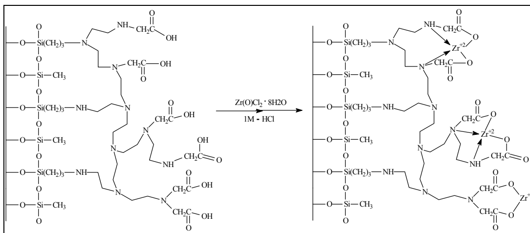
Figure 3.14: Schematic representation of the immobilization of \text{Zr}^{4+} on WP2.
