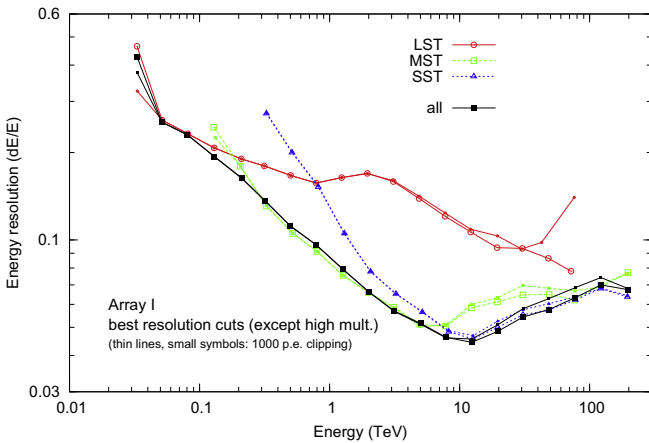
Fig. 11. Relative r.m.s. energy resolution \sigma(E)/E of array I as a function of energy (lines and symbols as in Fig. 9). Cuts were optimized for energy resolution, at a minimum multiplicity between two and six.
