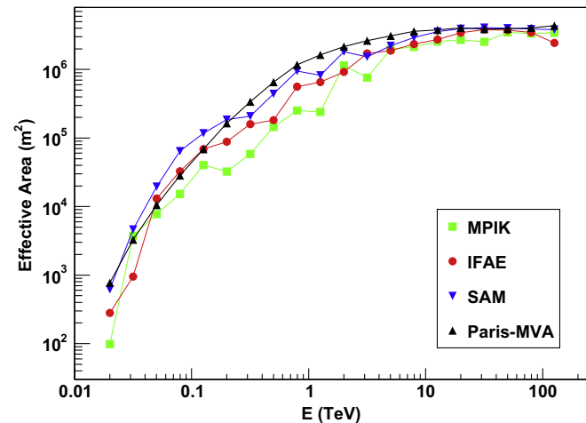
Fig. 15. Effective area of candidate array I, given as a function of the estimated energy for the baseline/MPIK (green squares), IFAE (red circles), SAM (blue triangles) and Paris-MVA (black triangles) analyses. The differential sensitivities are optimized for an observation time of 50 h. (For interpretation of the references to color in this figure legend, the reader is referred to the web version of this article.)
