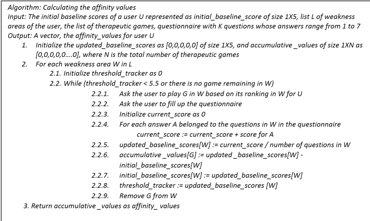
Figure 5.1: Algorithm 2. Calculation of affinity values
