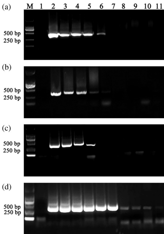
Fig. 2. Sensitivity of second round of nested PCR for each cDNA. M: DL2000 marker (TaKaRa); lane 1: healthy control; lanes 2–11: diluted to 10^{-10} dilution. (a) Oligo-dT; (b) random hexamer primers; (c) mixture of oligo-dT and random hexamer primers; (d) gene-specific primers.
