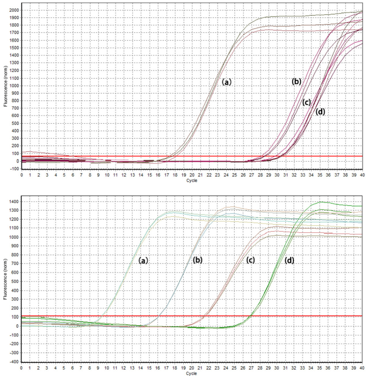
Fig. 4. Quantitative and nested qPCR amplification curve of four different methods. (top) Quantitative PCR; (bottom) nested qPCR. cDNA from (a) gene-specific primer; (b) mixture of oligo-dT/hexamer primers; (c) hexamer primer; (d) oligo-dT primer.
