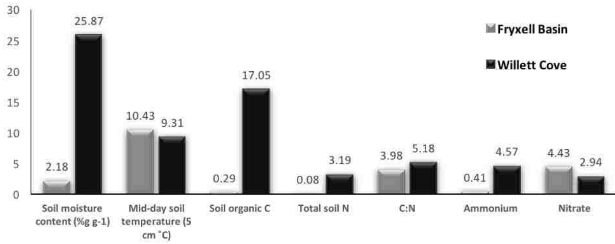
Soil habitat suitability of Scottnema lindsayae and Plectu murrayi
