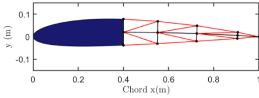
Fig. 4. Tensegrity topology of airfoil NACA2412 with shape error bound \delta = 0.001 m, along the chord 0–0.4 m (the shaded blue area) is ‘Rigid Structure’, and 0.4–1 m (the black and red lines) is ‘Flexible Structure’. (For interpretation of the references to color in this figure legend, the reader is referred to the web version of this article.)
