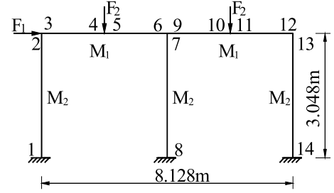
Fig. 7. A one-story two-bay frame.
