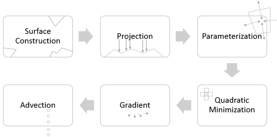
Figure 1: Algorithm Overview
