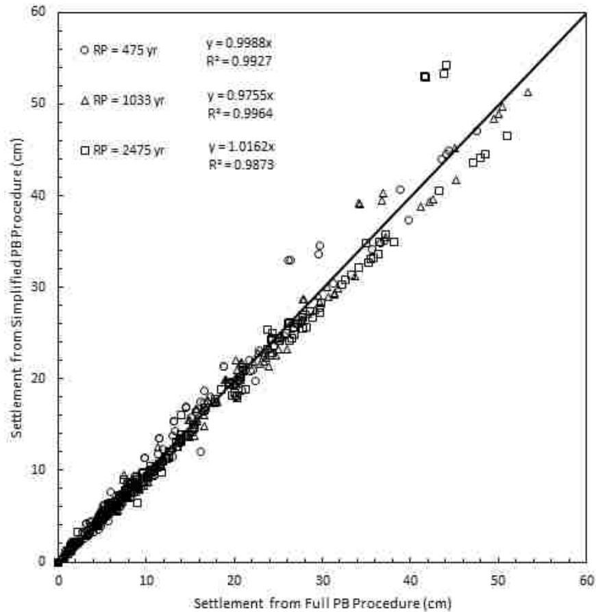
Figure 8-3: Boulanger and Idriss (2014) Full Performance-Based Settlement vs. Simplified Settlement Separated by Return Period (for PGA higher than 0.2g).
