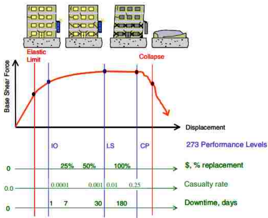
Figure 5-1: A Visualization of Performance-Based Earthquake Engineering (Moeble and Deierlein, 2004).
