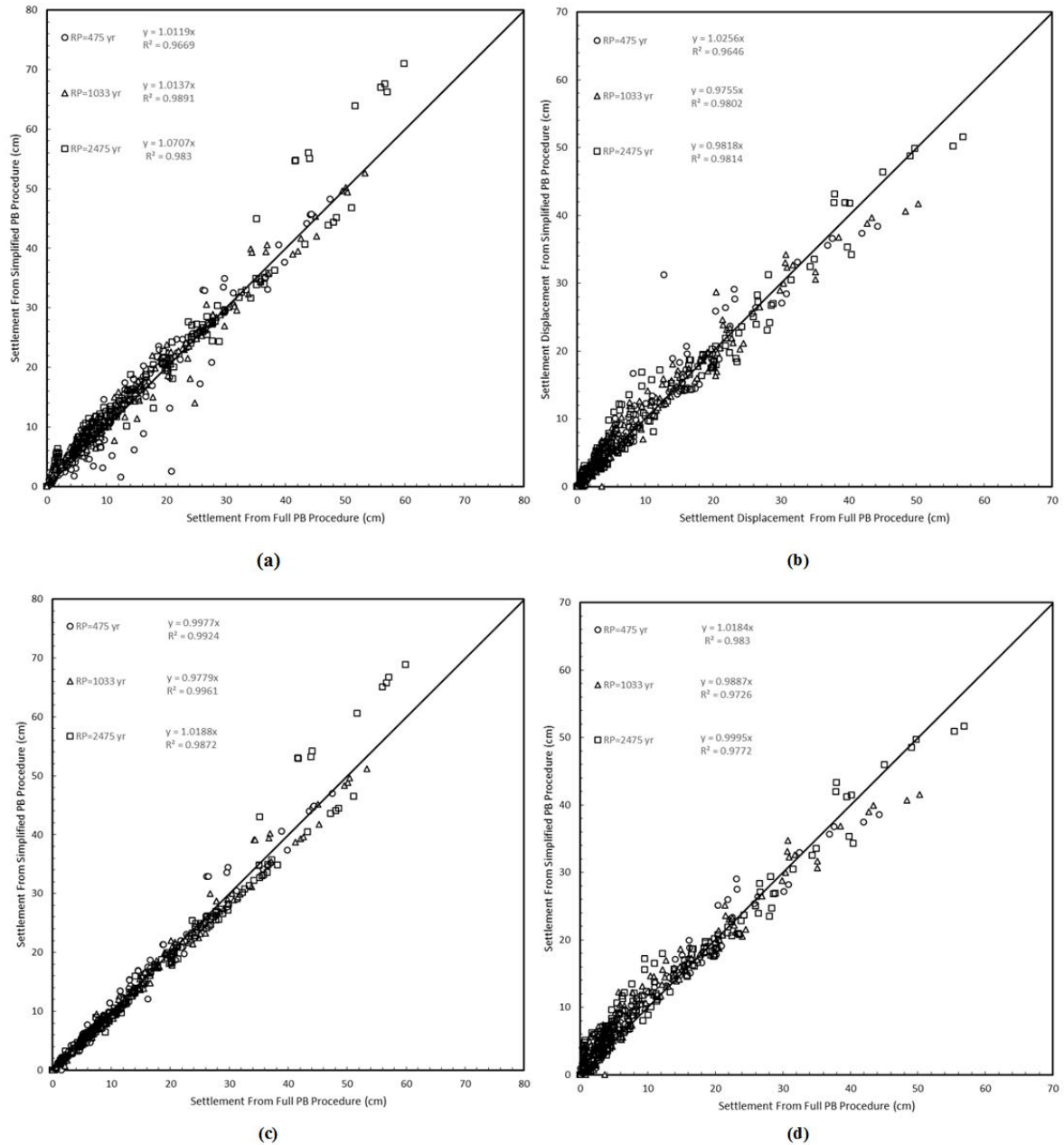
Figure 8-6. Comparative Scatter Plots for Simplified and Full Performance-Based Procedures Using (a) Semi-Probabilistic Results for B&I (2014), (b) Semi-Probabilistic Results for Ku (2012), (c) Pseudo-Probabilistic Results for B&I (2014) and (d) Pseudo-Probabilistic Results for Ku (2012) to Estimate the Correction Factor.
