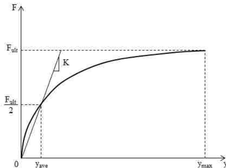
Figure 2-8: Shamsabadi et al. (2007) hyperbolic passive force-deflection curve
