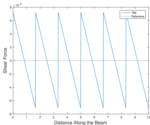
Figure 1.4: The calculated shear force for p = 1 .
