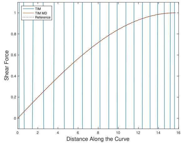
(c) Normalized shear force with p = 4 and \frac{R}{t} = 1000
