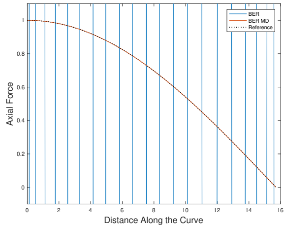
(c) Normalized axial force with p = 4 and \frac{R}{l} = 1000
