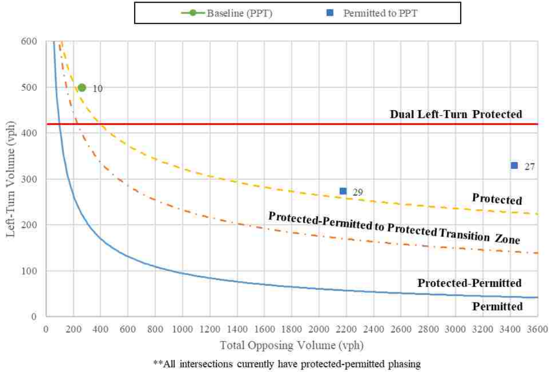
Figure 5-22: Existing 3-lane intersections outside of the proposed decision boundaries for 2- and 3-lane opposing approach configurations.
