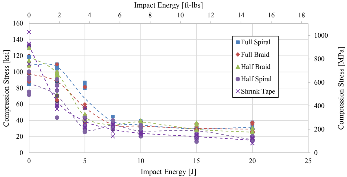
Figure 7.4 Compression Strength vs. Impact Energy for All Sleeve Types
