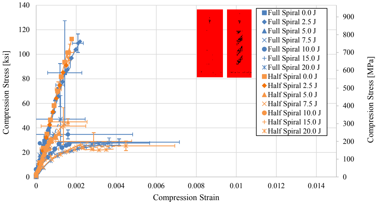
Figure 6.17 Average Stress-Strain Curves for Spiral Specimens
