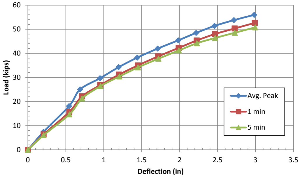
Figure D-1: Load-deflection curves for the 5.2D test.
