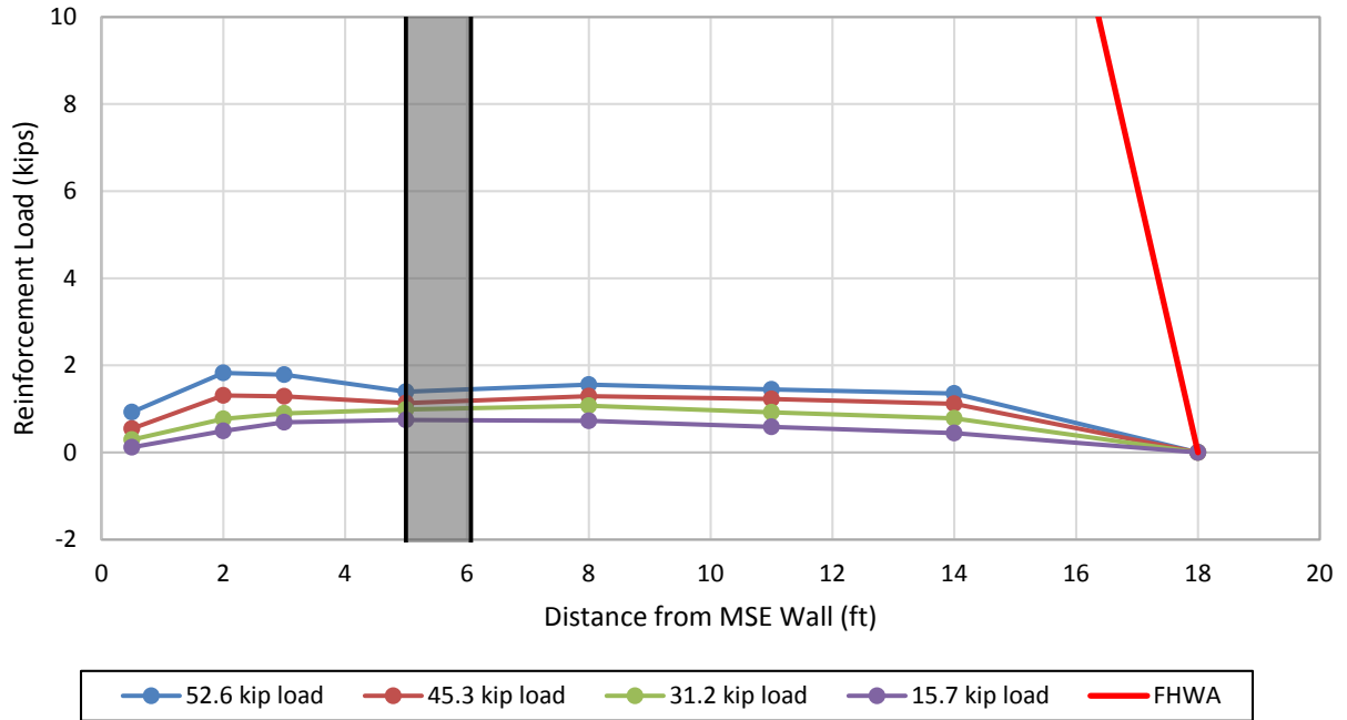
Figure F-1: Induced loads in the soil reinforcement at different pile head loads relative to distance from the back of the MSE wall (5.2D pile, layer L1, 46.5 in. transverse spacing).
