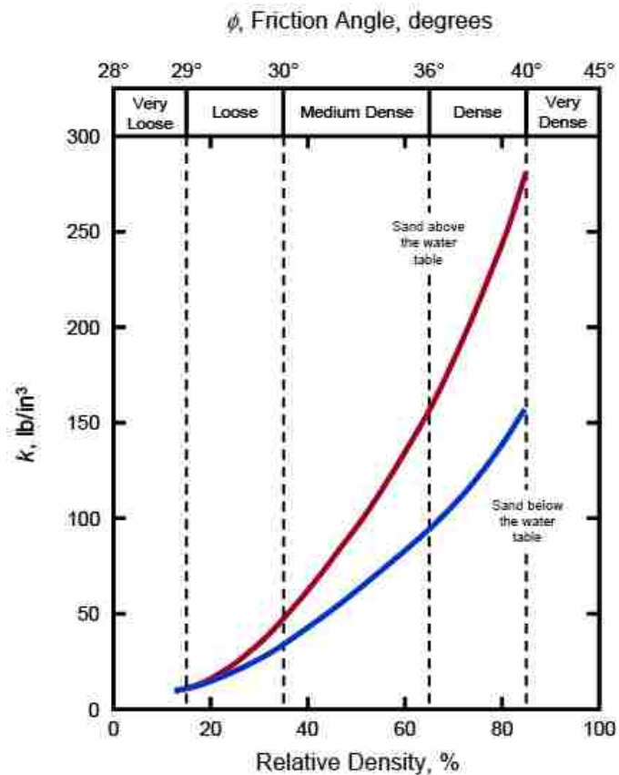
Figure 2-8: Soil modulus reaction based on friction angle or relative density of soil (API, 1982).
