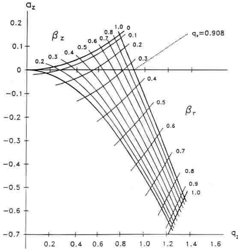
Figure 1-3: Stability diagram in a_z , q_z in the z-direction of 3D quadrupole ion trap. (Adapted from March, R. E., An introduction to quadrupole ion trap mass spectrometry. J. Mass Spectrom. 1997, 32, 351-369)
