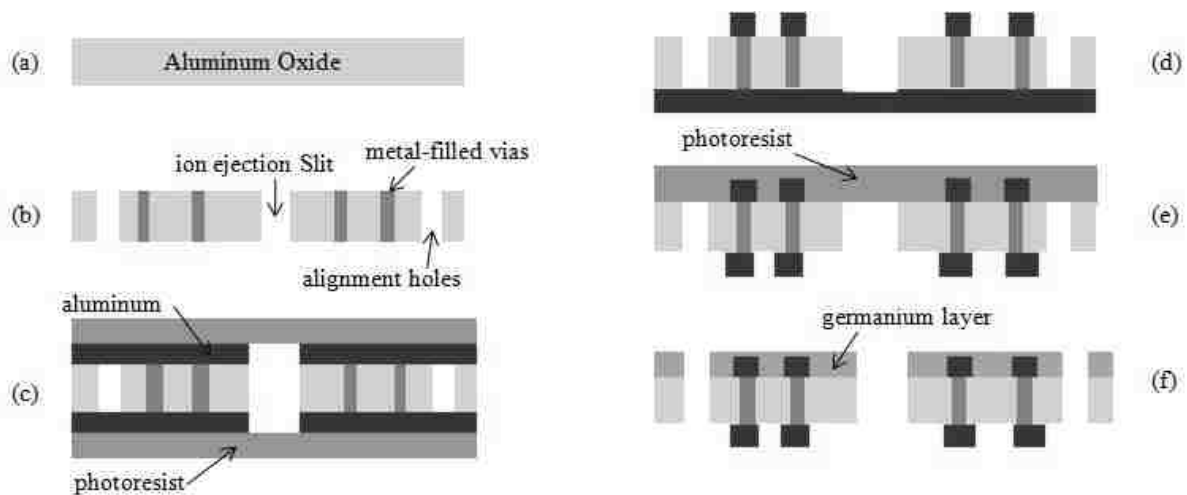
Figure 1-6: Cross-section view of the fabrication steps for planar electrode surfaces. (a) bare aluminum oxide substrate, (b) ejection slit, alignment holes, and metal-filled vias made by Hybrid-Tek (Clarksburg, NJ), (c) aluminum deposited on both sides of substrate, photoresist spun on top side and painted on bottom side, (d) top side patterned by photolithography and aluminum etching, (e) photoresist spun on bottom side, photoresist painted on already-patterned side, and bottom side is patterned and etched, (f) germanium layer deposited over top of trapping side of substrate. (Adapted from Hansen B.J.; Niemi, R.J.; Hawkins, A.R.; Lammert, S.A.; Austin, D.E. A lithographically patterned discrete planar electrode linear ion trap mass spectrometer. J. Microelectromech. Syst. 2013, 22, 876.)
