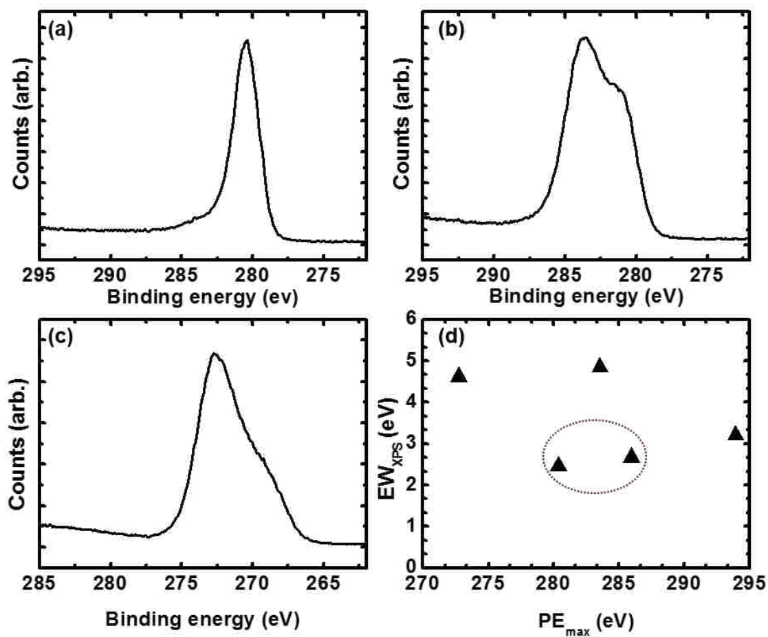
Figure 3.8 XPS C1s narrow scans of nanodiamonds that (a) showed a reasonable peak envelope, and (b – c) showed artifacts due to non-uniform charge compensation. (d) Graph of the EW XPS vs. PE max values from the C 1s narrow scans of five nanodiamond samples. The red dotted line is a guide to the eye.
