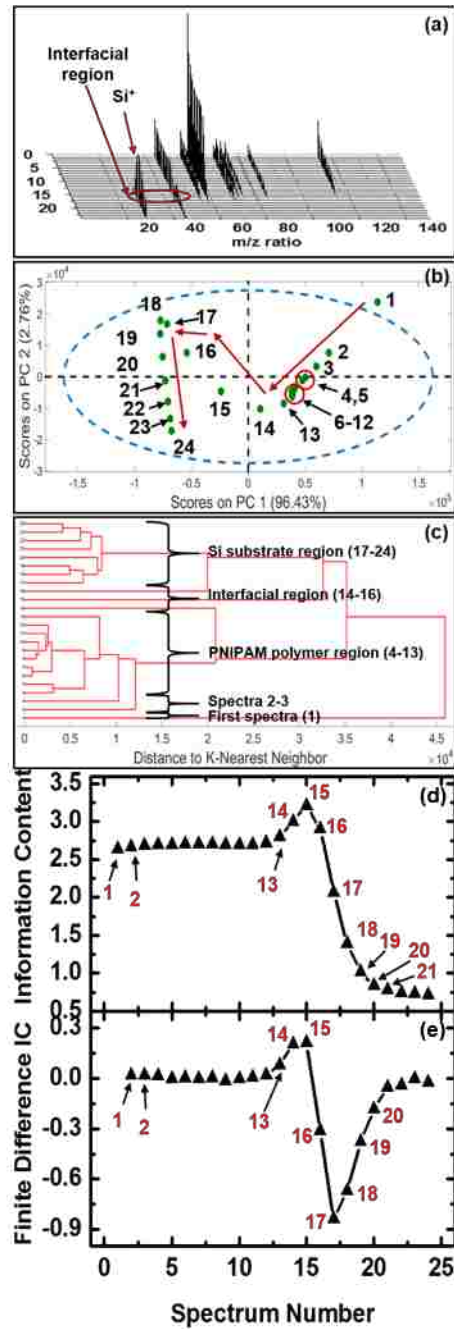
Figure 6.11 ToF-SIMS depth profiling study of PNIPAM/Si substrate: (a) 3-D graph of all 24 ToF-SIMS positive ion spectra, (b) scores plot of PCA analysis on the data, (c) cluster analysis on the data set, and (d) IC values and (e) finite difference IC as a function of spectrum number.
