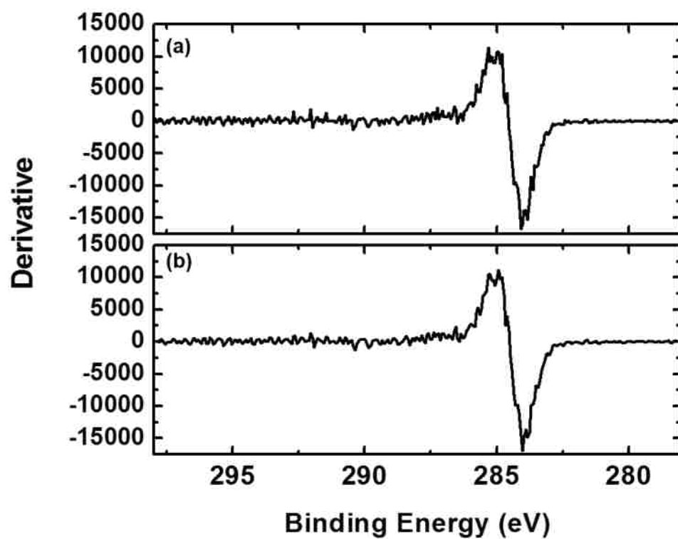
Figure 3.4 Derivative of the C 1s narrow scan of CNT Sample 1 using (a) the definition of derivative and (b) the five-point formula given in the text.
