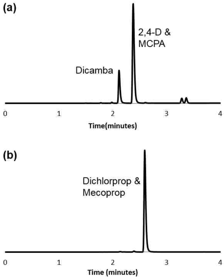
Figure A3. 3 (a) Attempted separation on a commercial PFP column of (a) MCPA, 2,4-D, and dicamba, and (b) dichlorprop and mecoprop. See Separation Conditions 2 below.
