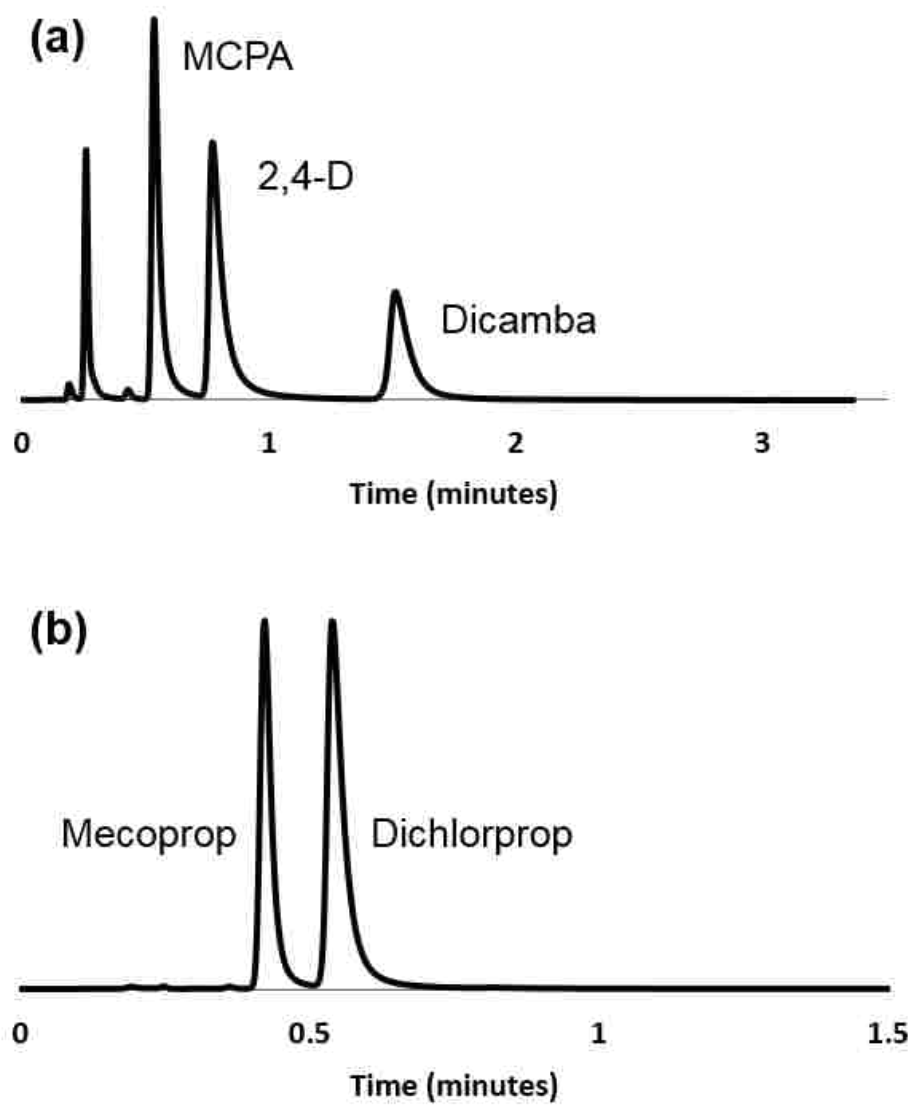
Figure A3. 4 Separation on a Diamond Analytics Flare mixed-mode column of (a) MCPA, 2,4-D, and dicamba, and (b) dichlorprop and mecoprop. See Separation Conditions 3 below.
