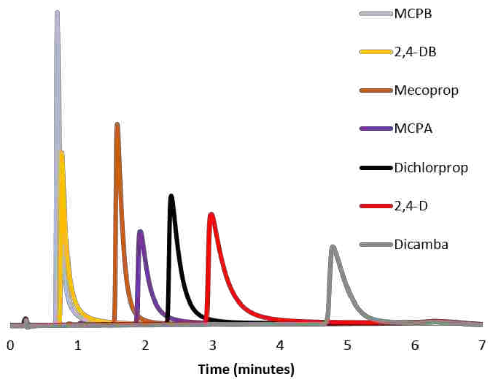
Figure A4. 2 Separation of acidic herbicides on the Flare mixed-mode column.
