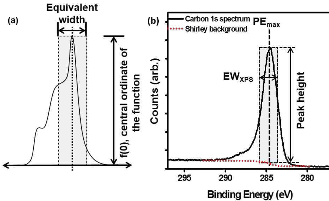
Figure 3.1 Graphical illustrations of (a) the EW of a general function, f(x) , and (b) the EW_{XPS} of a C 1s XPS narrow scan calculated with respect to a user defined baseline.
