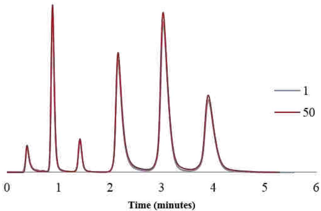
Figure A5. 3 Chromatograms corresponding to the 1 st and 50 th injections of the test mixture on the Flare column.
