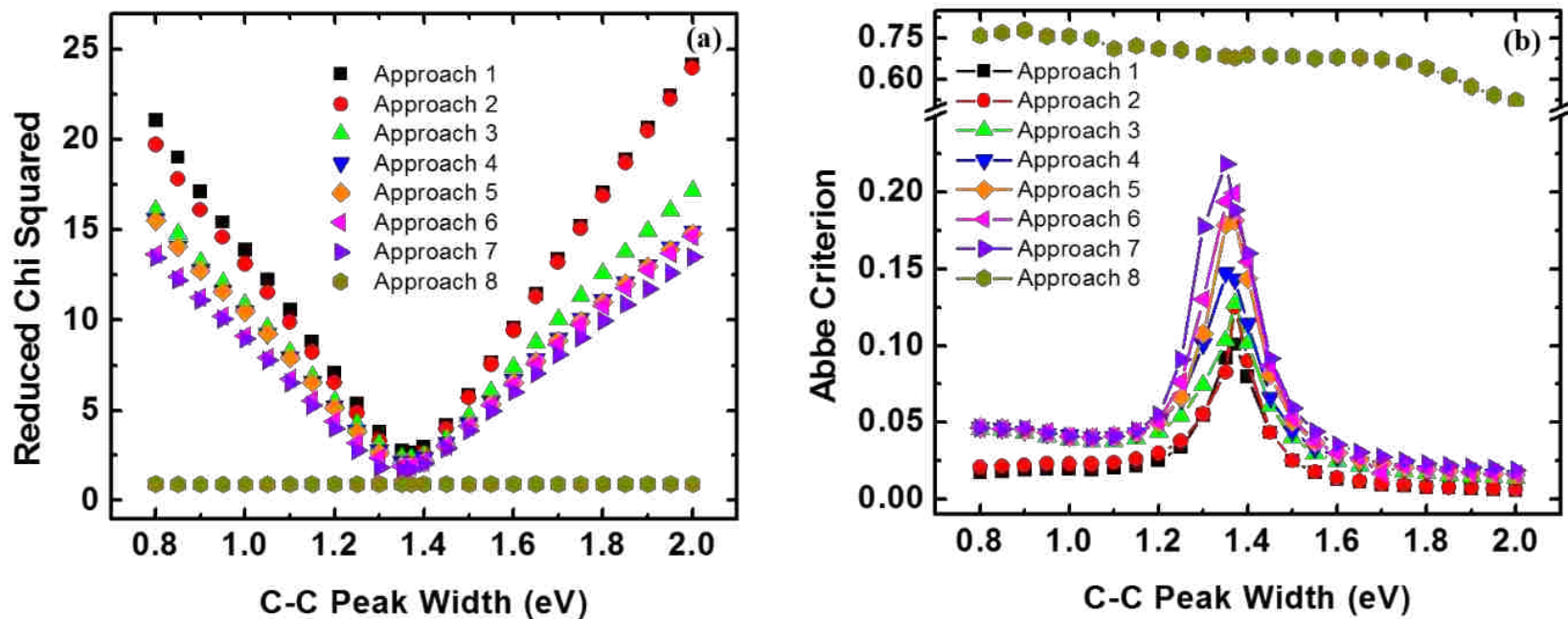
Figure 5.3 Uniqueness plots for the fits to a C 1s narrow scan of ozone-treated CNTs using the eight approaches described in Table 5.1. See also Figures 5.2 and 5.4. Plots of (a) reduced chi squared and (b) the Abbe criterion value vs. a fit parameter (the C-C peak width) that was fixed to specific values.
