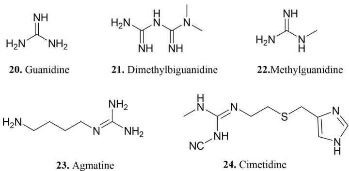
Figure 8 Guanidine compounds.
