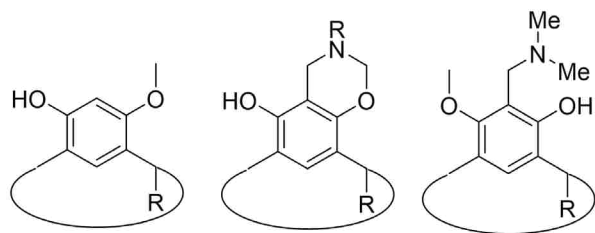
Figure 5 Inherently chiral C_4 -symmetric resorcinarenes. 30
