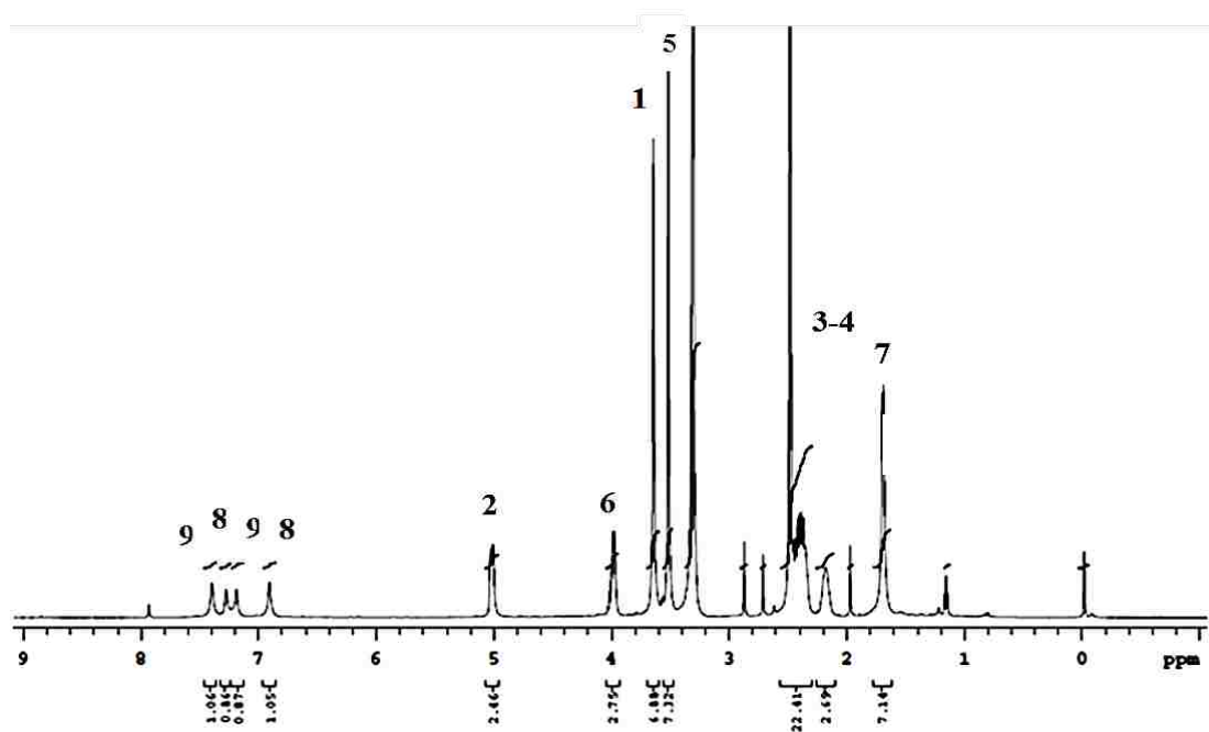
Figure 6 ^1\text{H} NMR of GME in d_6 -DMSO.
