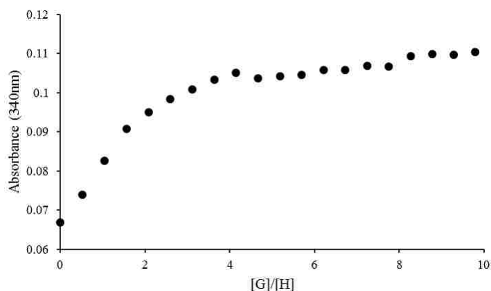
Figure 9 UV-vis absorbance change with added 23 to GMA. Adding guest 23 to the 0.0360 mM of GMA and monitoring the peak shift at 340 nm. The absorbance at 340 nm is plotted vs the [guest 23]/[host] concentration.
