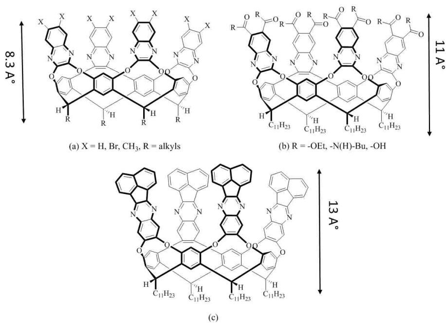
Figure 3 The structure of deepened cavitants, a : bridging with 6,7- disubstituted-2,3- dichloroquinoxaline, b ) elongated with a reaction of octanitrocavitant with phenylenediamine units and condensed with 1,2-diketones c ) bridging with acenaphthenequinone. 21,22
