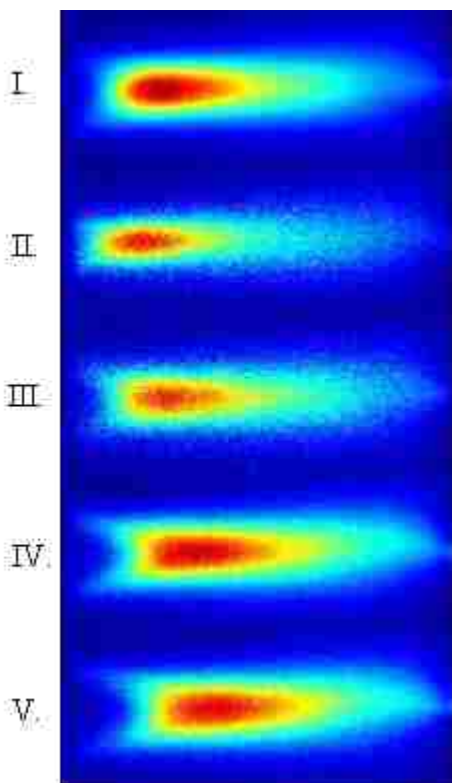
Figure 2.5 LIF images showing the influence of solvent on Sc ion densities in the ICP. In each image, 1.0 \text{ L mm}^{-1} of Ar was split equally between the LA and SN systems. Image (I) was obtained while aspirating 50 ppm Sc without LA aerosol. Images (II) and (III) were obtained during LA at 28 \text{ J cm}^{-2} without and with aspirating 2% nitric acid, respectively. Images (IV) and (V) were identical to (II) and (III) but performed at 60 \text{ J cm}^{-2} . Due to the significant difference in the signal intensities of each image, the color scales for each image are different.
