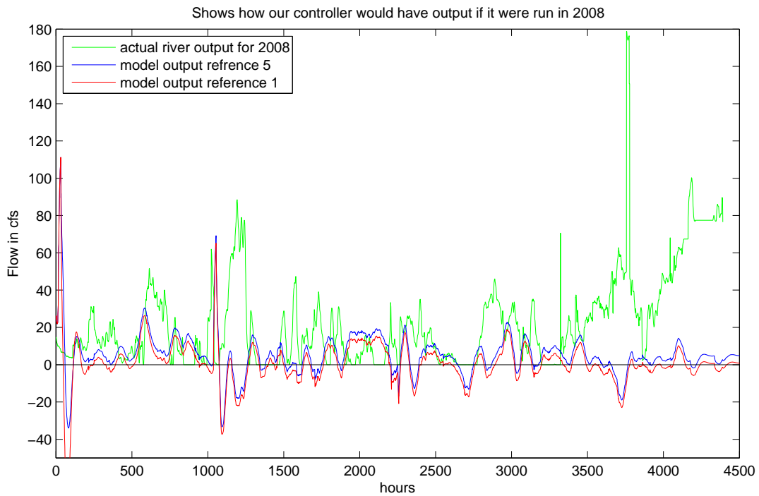
Figure 4.16: Actual river output (green) compared with system output with the controller actuating the reservoir release. The controller was given a reference signal of 1 cfs (red) and 5 cfs (blue) to try and maintain. The controller saves water but also may cause a canal to not get enough water because it goes below zero several times.
