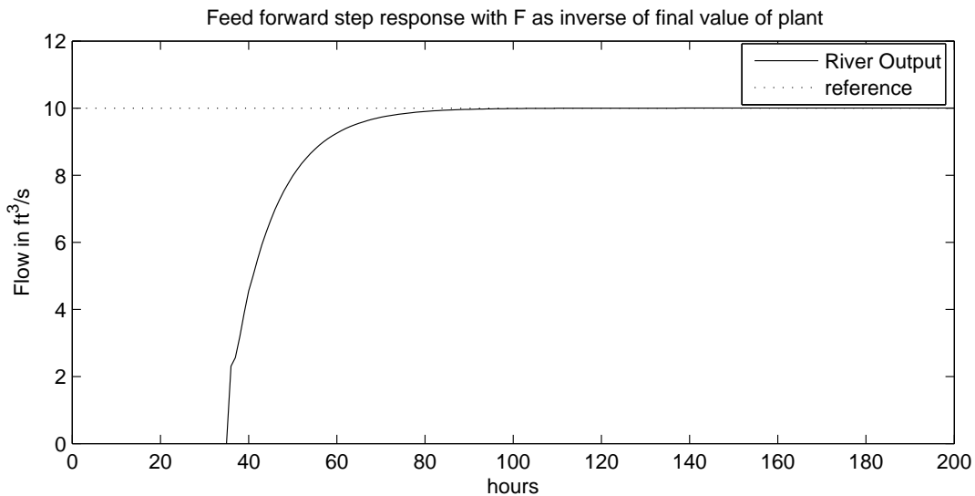
Figure 4.7: Open loop system with the feed forward controller. The plant is the model developed in the previous section and the feed forward controller has gain equal to 2.426. The system is stable and tracks steps in the reference command.
