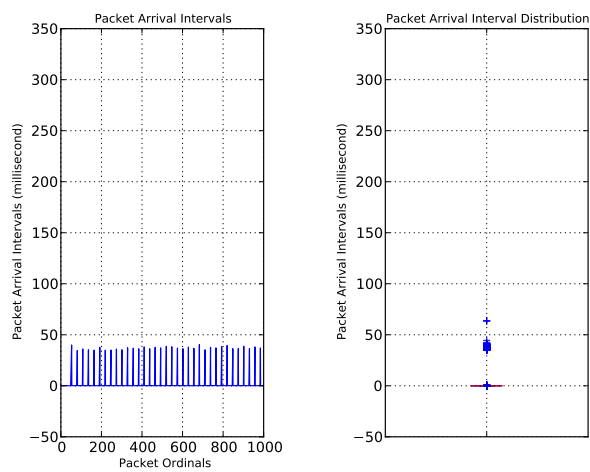
Figure 8.7: Outgoing packet arrival intervals at node 25
