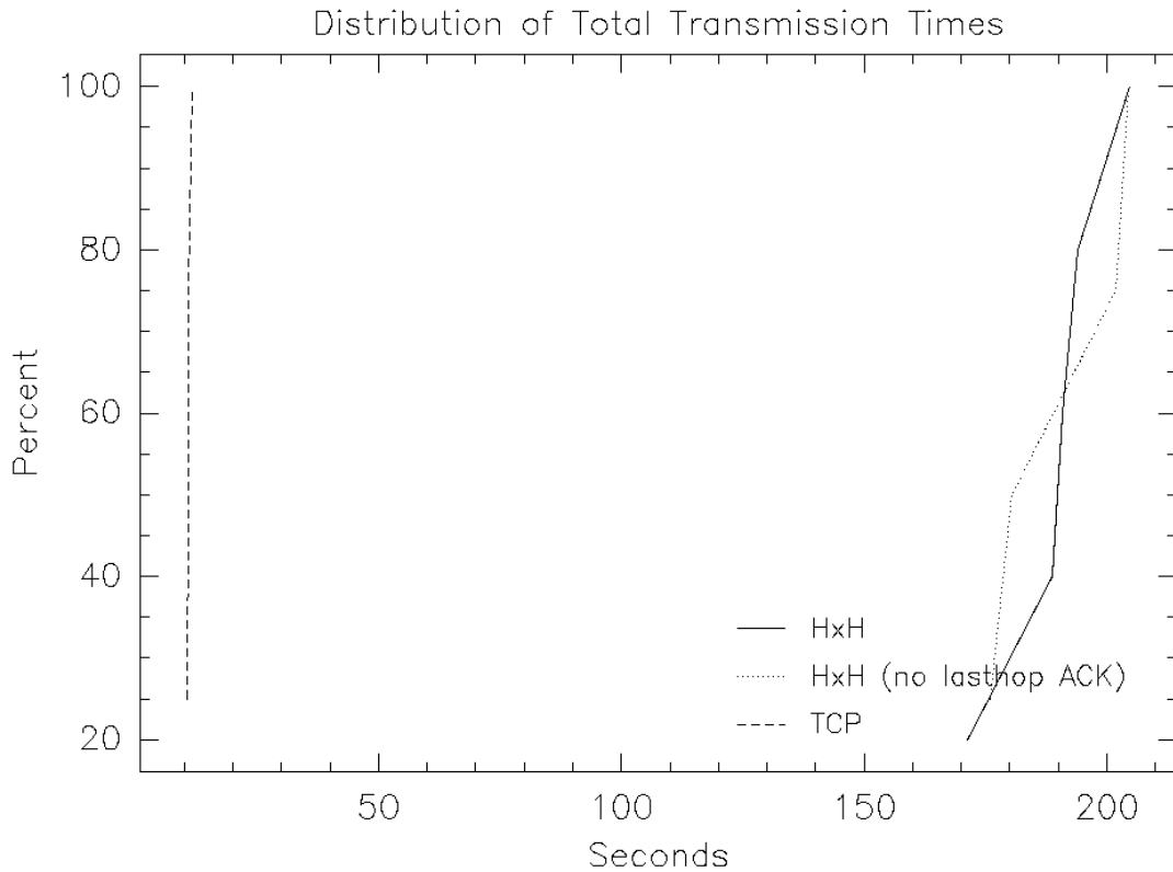
Figure 5.6: Throughput from mesh8 through mesh9, mesh1, mesh4, mesh2, mesh5, mesh7, and mesh6 to mesh3: This graph shows the cumulative distribution function of the times taken to transfer one megabyte from mesh8 to mesh13 using TCP, HxH, and HxH without last hop acknowledgments using a buffer size of 8 packets.
