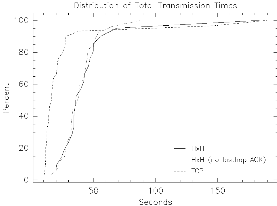
Figure 5.5: Throughput from mesh8 through mesh9, mesh1, mesh4, mesh2, mesh5, mesh7, mesh6, and mesh3 to mesh13: This graph shows the cumulative distribution function of the times taken to transfer one megabyte from mesh8 to mesh13 using TCP, HxH, and HxH without last hop acknowledgments.
