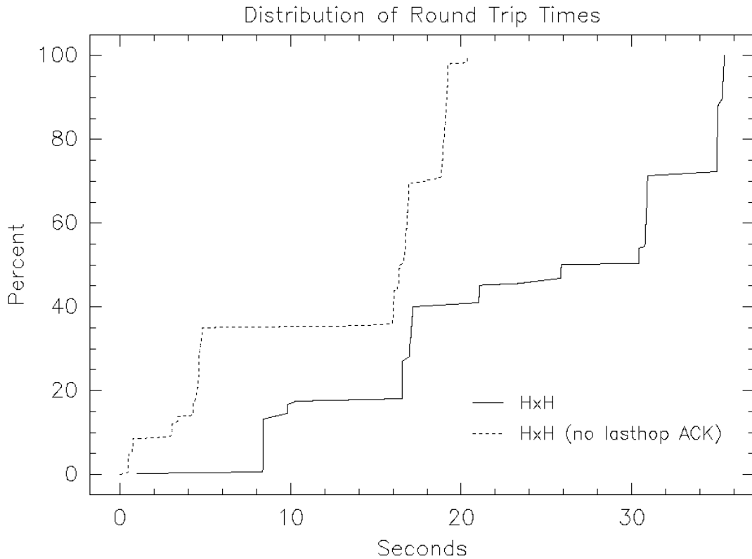
Figure 5.12: Round trip times from mesh6 through mesh5, mesh2, and mesh4 to mesh1 : This graph shows the cumulative distribution function of the intervals between the transmission of a packet from mesh6 to mesh1 and the receipt of a corresponding passive acknowledgment using HxH and HxH without last hop acknowledgments.
