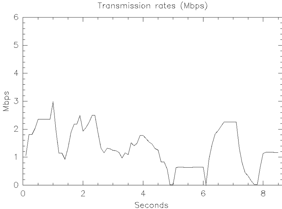
Figure 5.27: Transmission Rates at mesh8 over time for a transmission from mesh8 through mesh9, mesh1, mesh4, mesh2, mesh5, mesh7, and mesh6 to mesh3 : This graph shows the amount of data transmitted per second using a one-second sliding window plotted every 100ms. The transfer does not use last hop acknowledgments and uses a buffer size of 128 packets.
