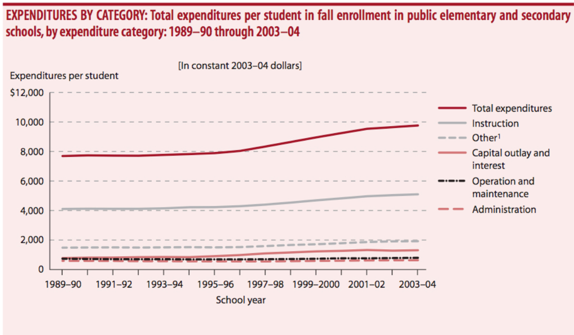
Figure 1. Total Student Expenditures
