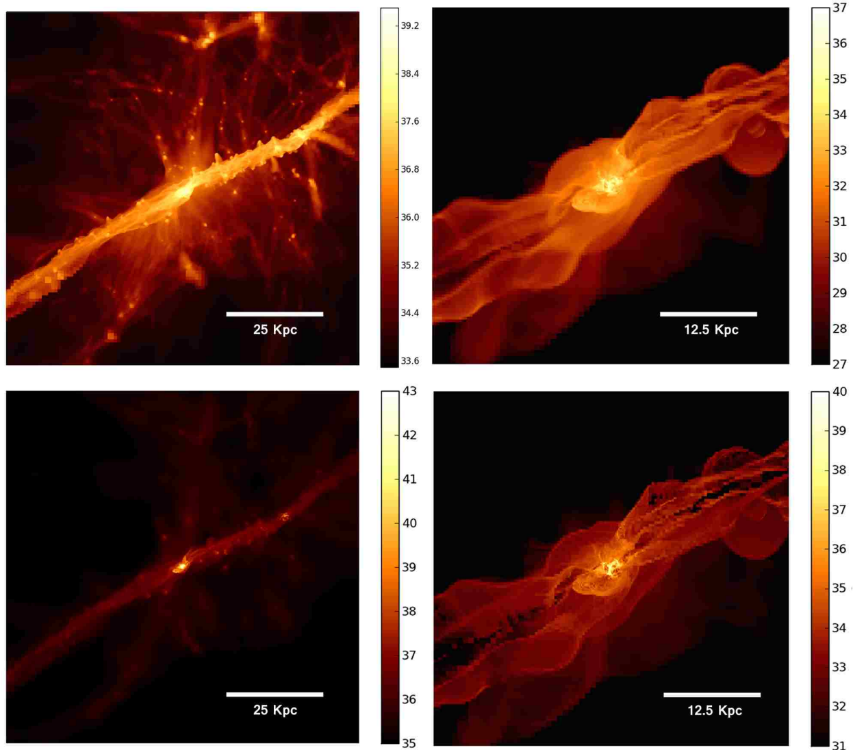
Figure 3.8 Projection of logarithm of emissivity [ \text{erg s}^{-1} ] in Lyman- \alpha (left panels) and HeII 1640 Å (right panels). In the top panels, we plot emissivity due to radiative recombination. In the bottom panels, we plot emissivity due to collisional excitations. Note the difference in color scales.
