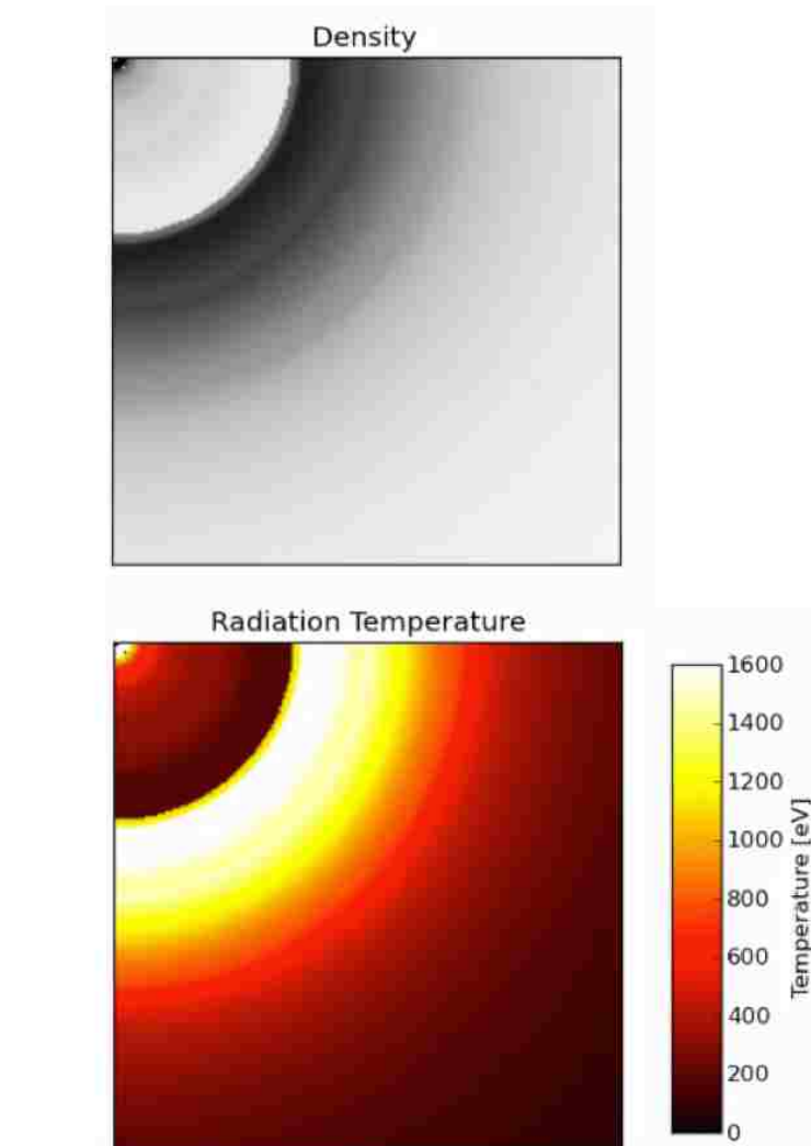
Figure 2.14 Snapshot of a RAGE hypernova simulation sometime following the moment when the shock-wave breaks through the surface of the star and plows through the ambient medium. RAGE simulations are carried out in one dimension, so the extra dimension visualized here serves only to emphasize structure and provide a feel for the phenomenon. In the upper panel, relative density is indicated, black being regions with the most material. At this stage, the star has been almost completely disrupted into a ring (or a sphere in three dimensions) of glowing material. Matter has fallen back onto the central black hole (upper lefthand corner), which is radiating as observed in the bottom frame. Note that though the scale bar in the lower panel only indicates temperature up to 1600 eV, regions of this panel are tens of thousands of eV.
