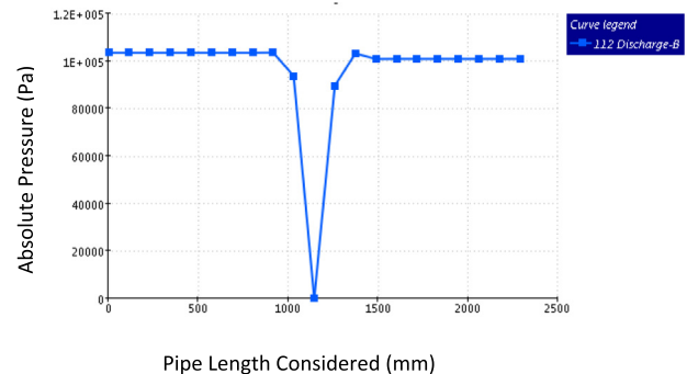
Fig. 5. Absolute pressure curve for 112 m 3 /h volumetric discharge rate.
