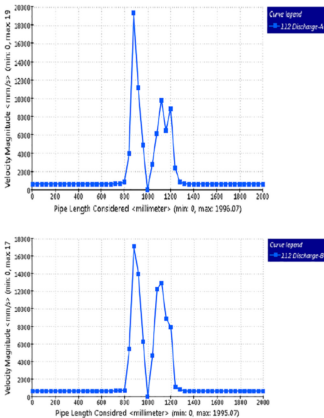
Fig. 7. Vorticity magnitude curve for 112 \text{ m}^3/\text{h} volumetric discharge rate.
