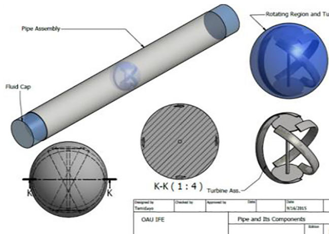
Fig. 3. In-pipe turbine assembly of rotating region.
