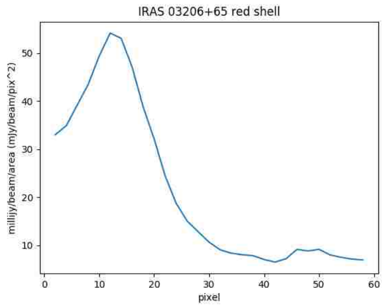
Figure 3.2 Radial plot of the 1612 MHz emission of IRAS 03206+6521 of the red shell region. Intensity in concentric rings is totaled then divided by the total area within the ring.
