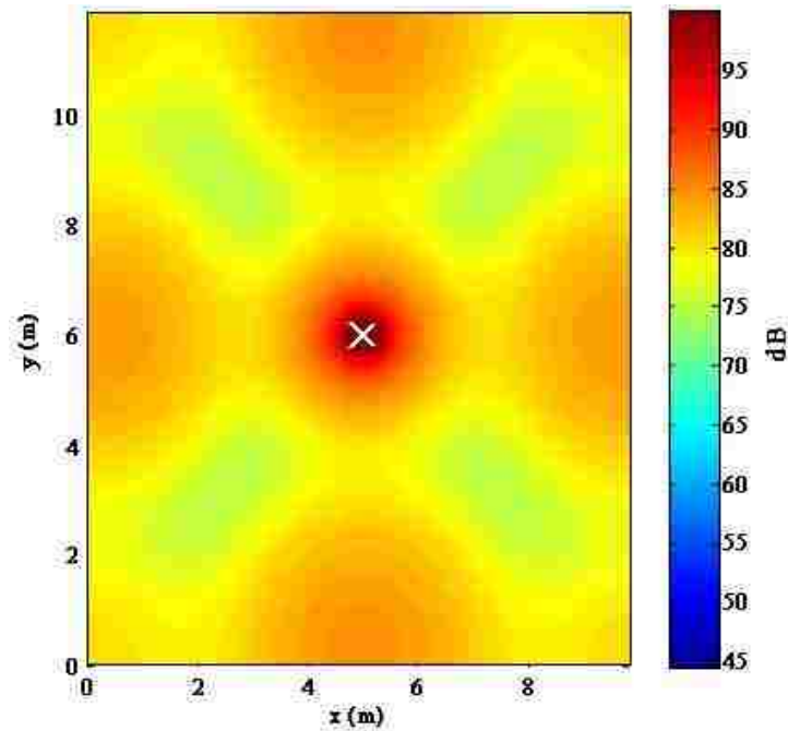
Figure 2.3 Plan view of the TED field produced by a point source radiating at 50 Hz in a rectangular enclosure of uniform absorption and dimensions 10 x 12 x 14 m. The absorption coefficient is 0.01 and the position of the source is indicated by the “X” symbol. The horizontal plane intersects the source located at x = 5 m, y = 6 m, z = 7 m. The complex impedance value of the boundaries is 200 + 340i .
