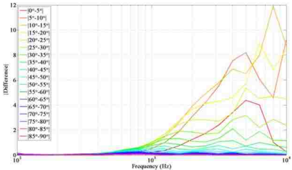
Figure 4.8 The absolute value of the difference between the directivity factors for each respective pair of angles [ Intended - Actual ], relative to the principal axis. These results are for the horn-loaded compression driver.
