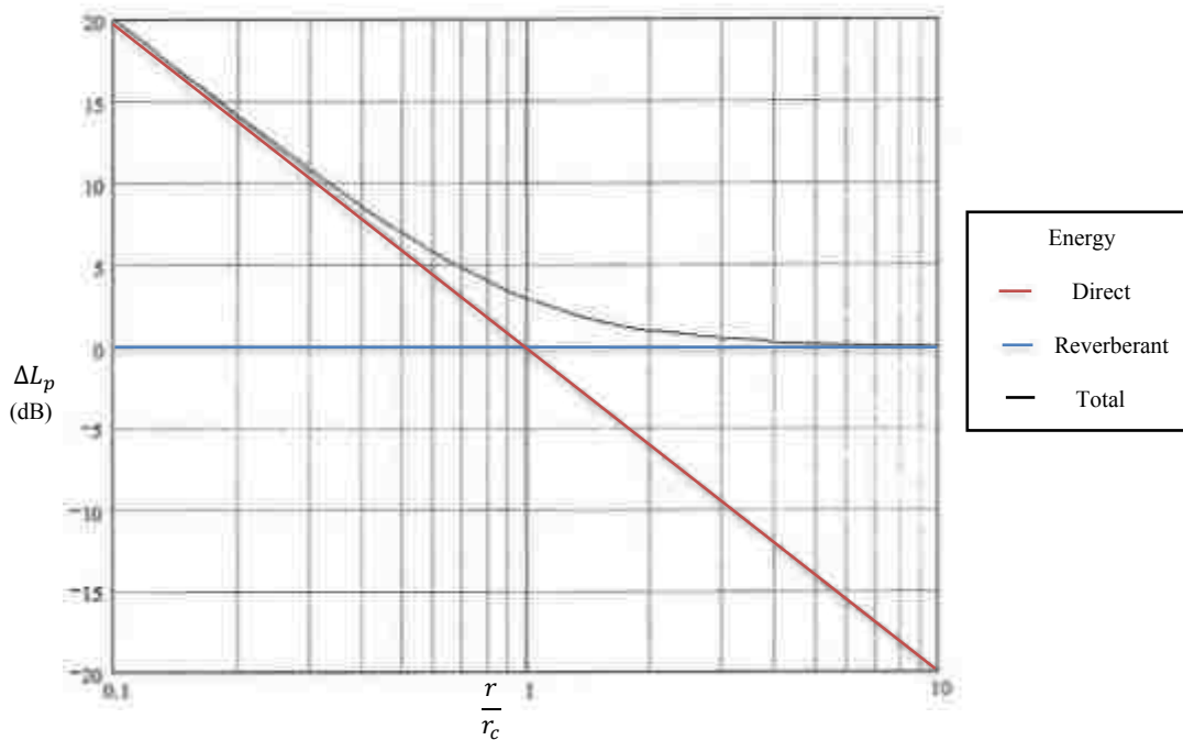
Figure 1.1 The change in sound pressure level \Delta L_p relative to that at the critical distance r_c for the direct, reverberant, and total energy fields as a function of distance r from the source. The critical distance is the radial distance for a given angle where the direct and reverberant energy values are equal.
