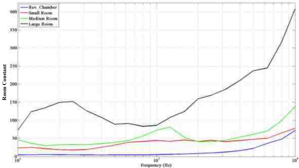
Figure 3.19 The 1/3-octave band room constant R for each of the four test environments.
