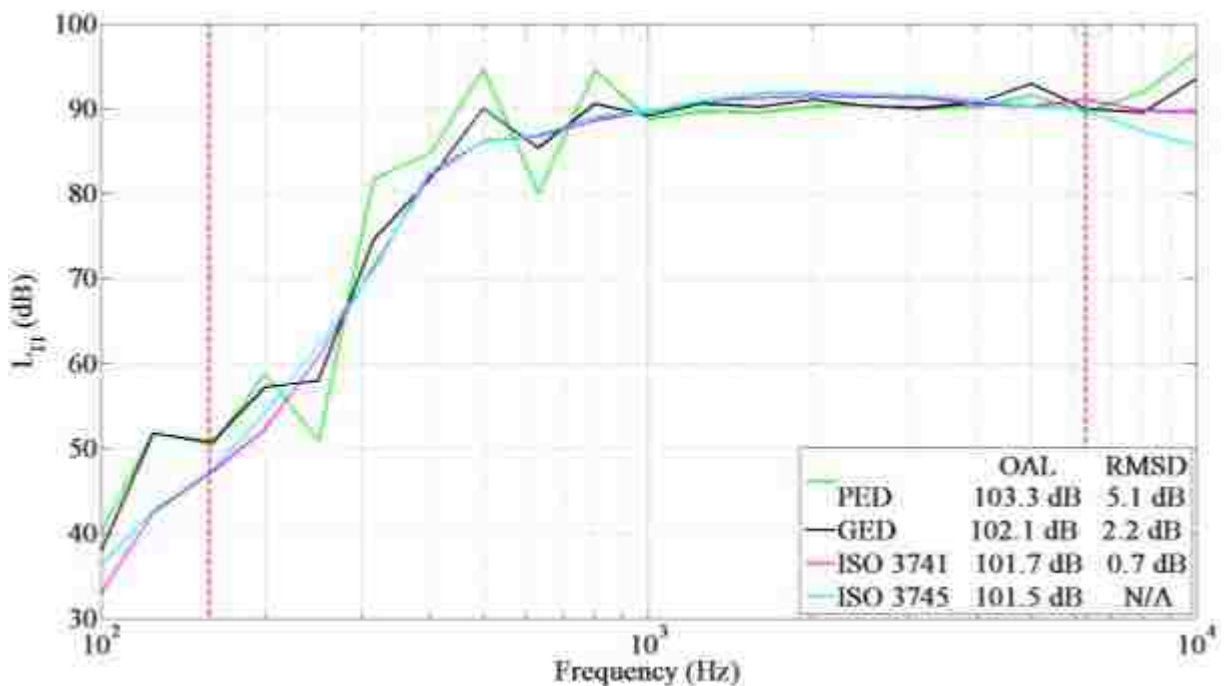
Figure 4.4 1/3-octave band sound power estimates of the horn-loaded compression driver calculated from the two-point in situ method, at 45° off axis, in the small room. The single-driver dodecahedron served as the reference directivity source and the energy density fields were measured by the G.R.A.S. Type 50VI. The RMSD results are compared to the reference power curve measured by ISO 3745.
