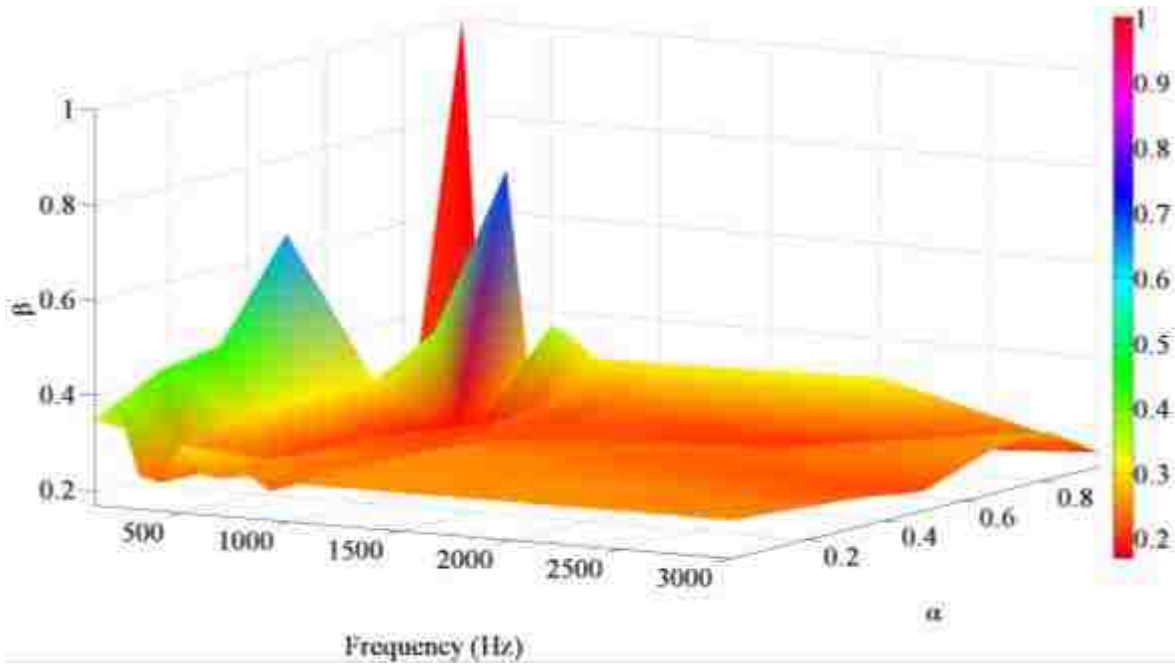
Figure 2.12 Surface plot of the GED weighting factor \beta as a function of frequency and room absorption coefficient \alpha , which minimizes the coefficient of variation of the GED field within an enclosure of dimensions 5 x 6 x 7 m.
