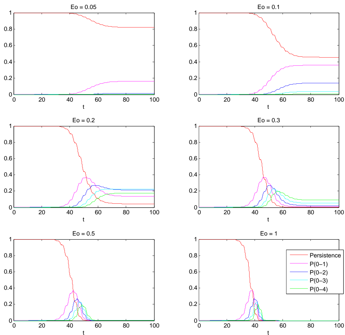
Figure 3.6 SHO transition probabilities, small E_0 values, \lambda = 0.005 , \omega_f = \omega .
