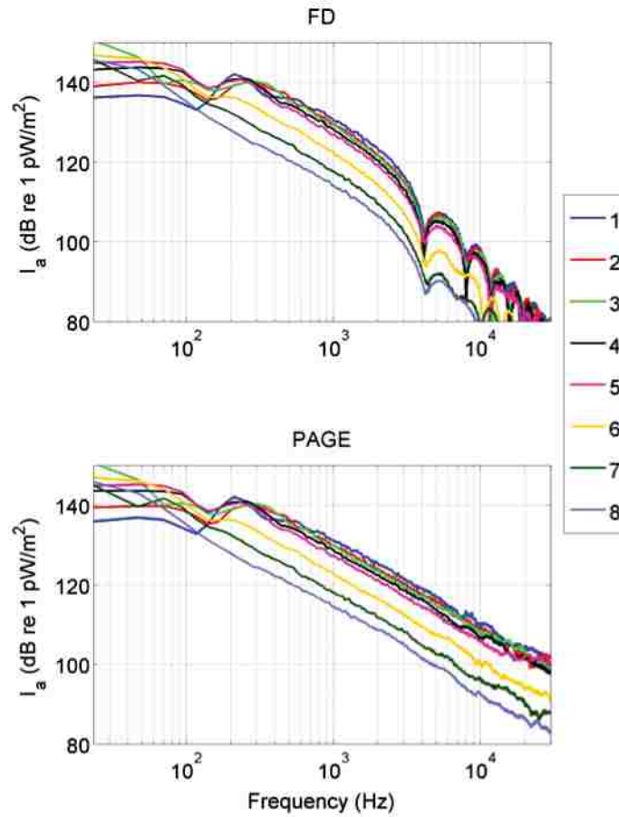
Figure 4.7: The active intensity magnitude estimated from the eight 2D intensity probes parallel to the shear layer. The probes are numbered from closest to farthest from the GEM-60 nozzle (see Fig. 4.1). The estimates calculated through the FD method are accurate up to approximately 1500 Hz, whereas the PAGE estimates appear to be accurate up to approximately 10kHz.
