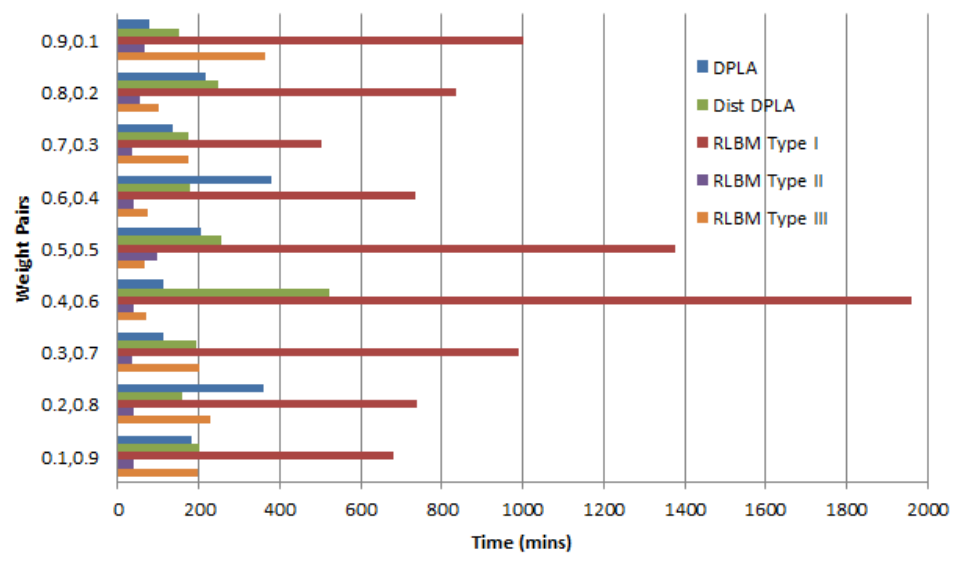
Figure 7.8. Time to Converge
