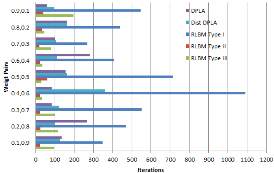
Figure 7.7. No. Of Iterations
