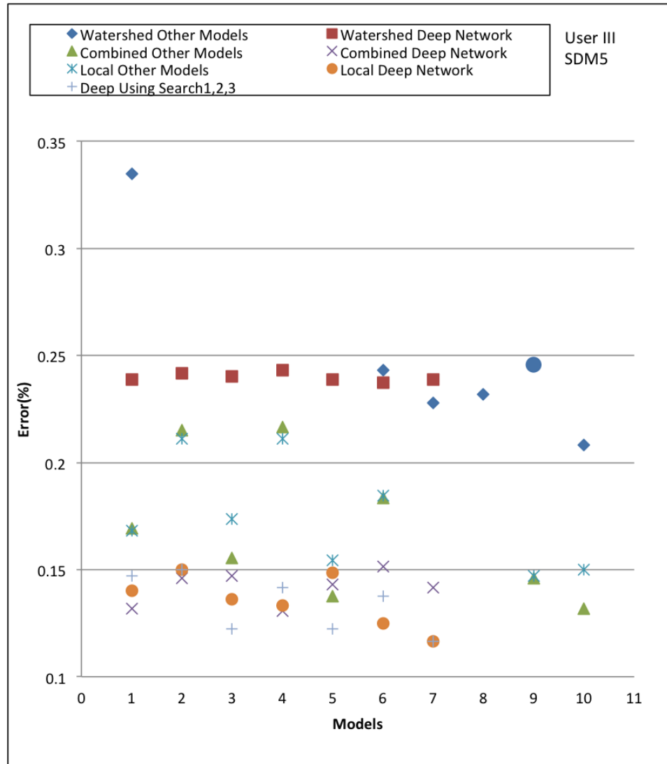
Figure 7.27. Deep Learning Result - User III
