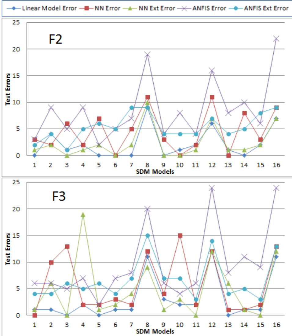
Figure 7.16. Mixed Rating Functions
