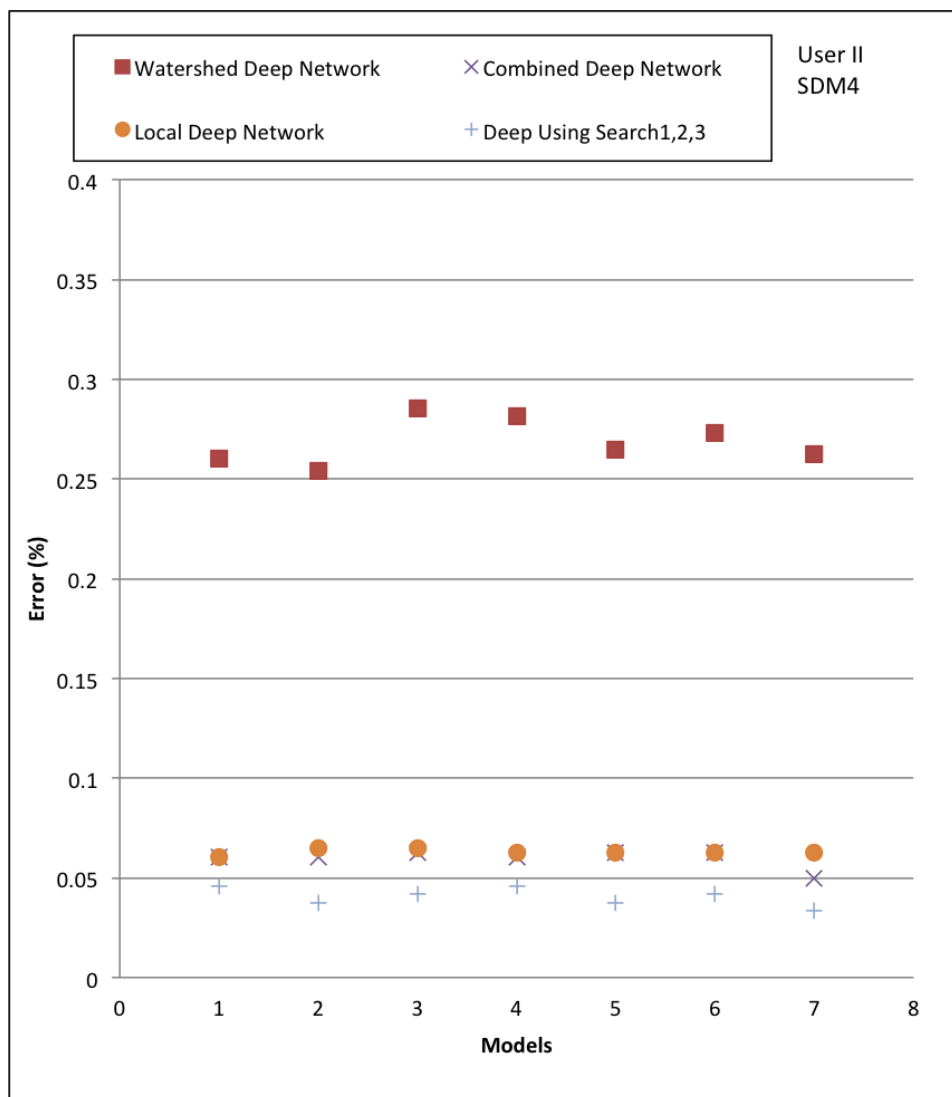
Figure 7.29. Deep Learning local decision Result - User II
