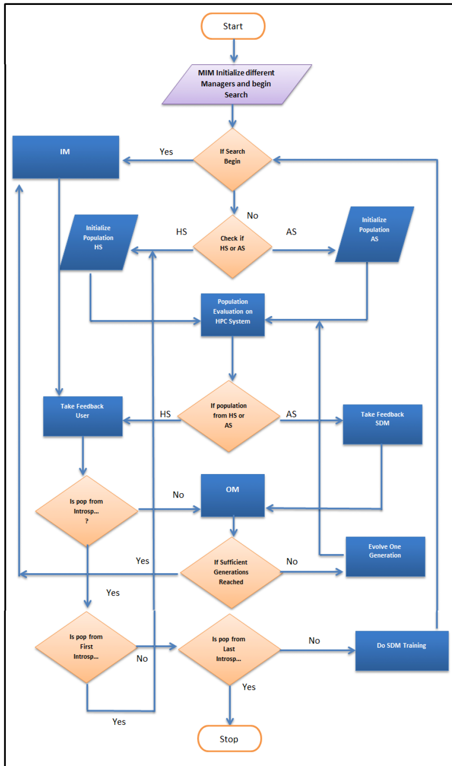
Figure 3.4. Flow Chart working of IGAMI2 Search and Learning
