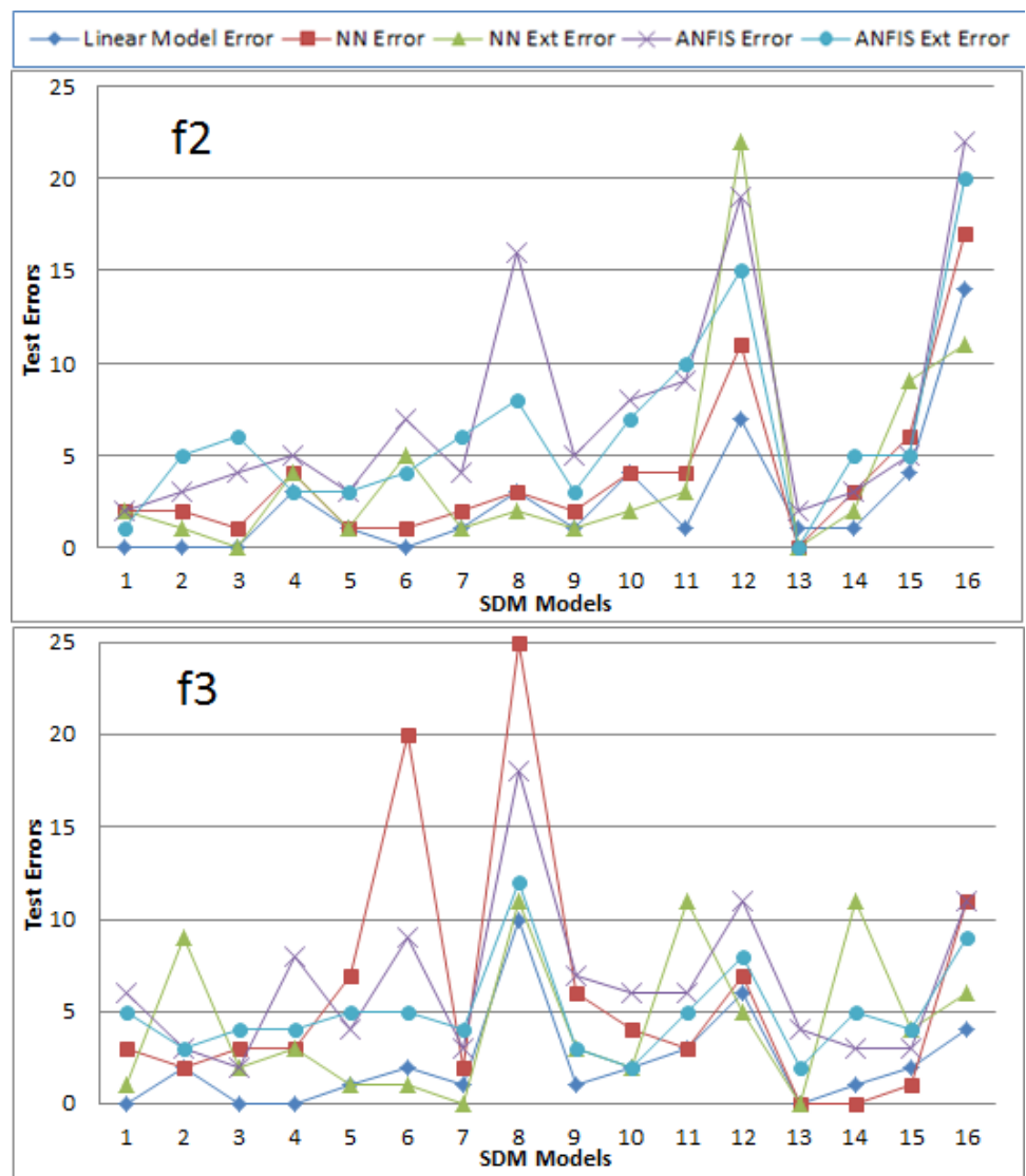
Figure 7.17. Simple Rating Functions
