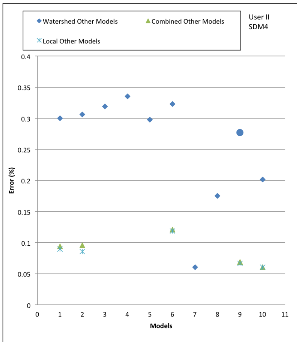
Figure 7.23. Local Decision Result - User II
