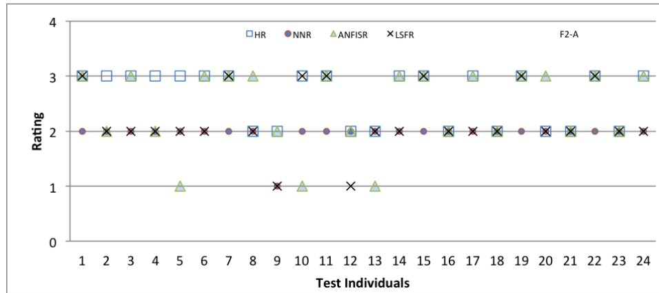
Figure 7.14. Simulated User with Rating F2
