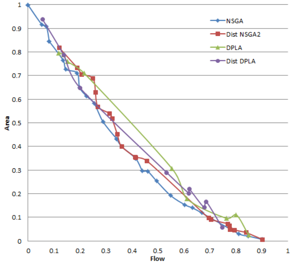
Figure 7.4. NSGA2 Vs DPLA
