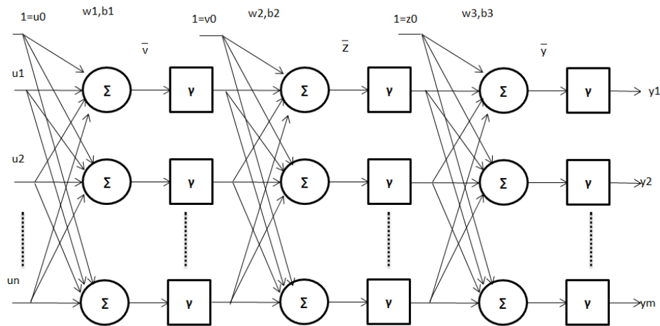
Figure 6.1. A Feed Forward Artificial Neural Network
