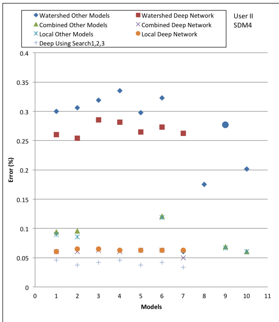
Figure 7.26. Deep Learning Result - User II
