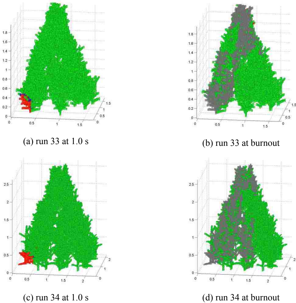
Figure 6.18. Bush combustion modeling results of run 33 and run 34.
