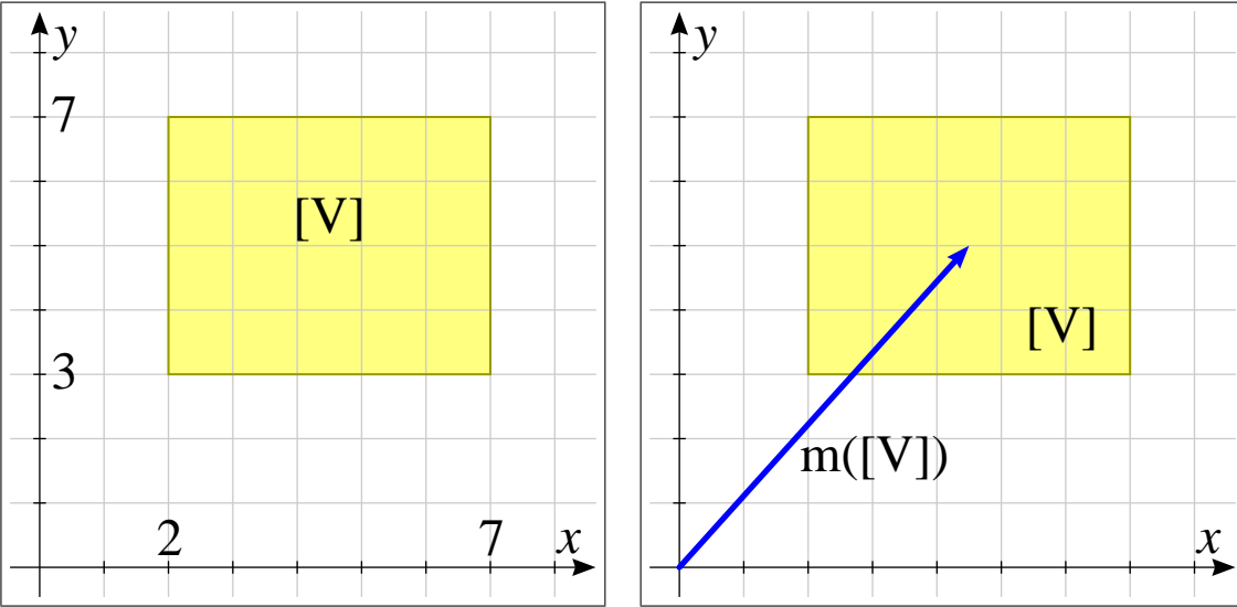
(a) The interval vector [V] = ([2, 7], [3, 7]) .
