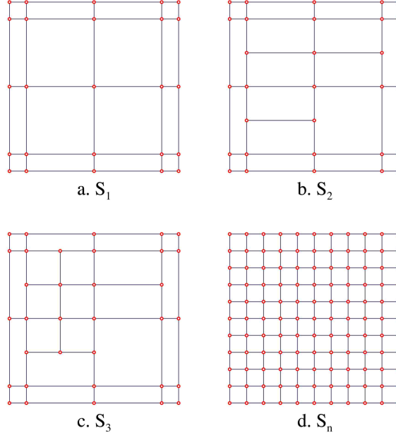
Figure 5.2: Nested sequence of cubic T-Spline spaces.
