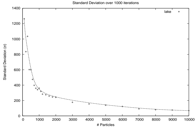
Figure 4.10: Standard Deviation in error estimates for the Lake dataset. We see that increasing the number of particles guarantees more consistent performance of the Particle Filter
