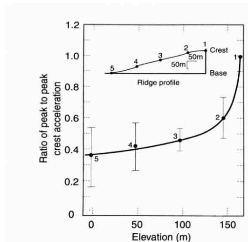
Figure 2-7: Normalized peak accelerations (means and error bars) recorded on mountain ridge at Matsuzaki, Japan (Jibson, 1987).
