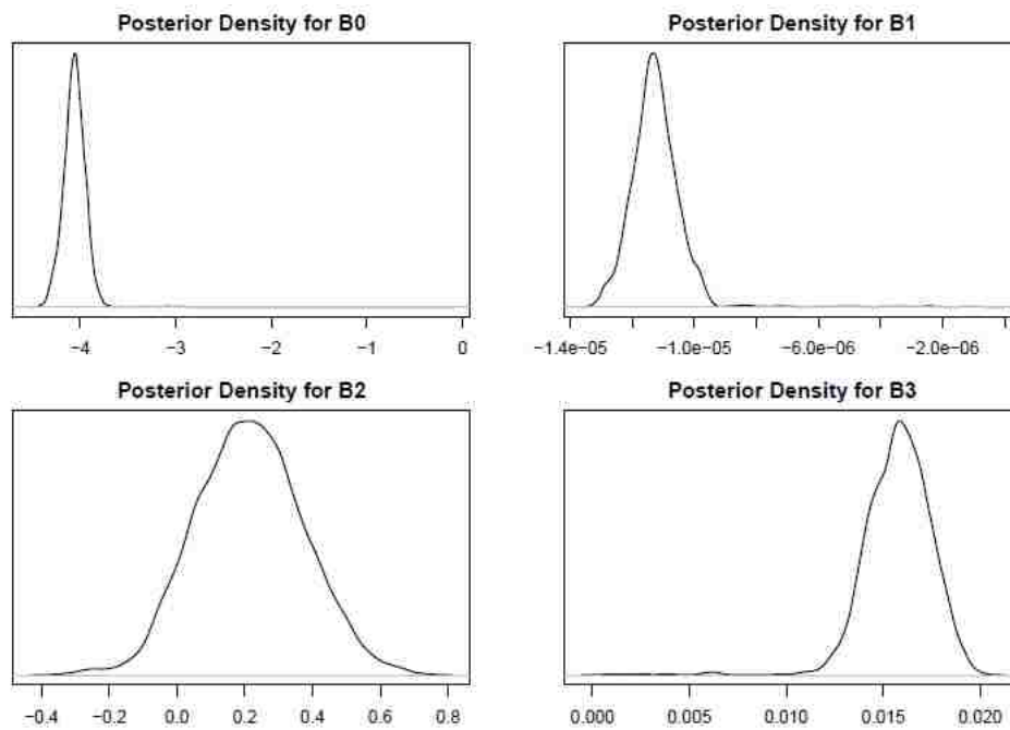
Figure 5-4: Example of posterior density plots from statistical analysis.
