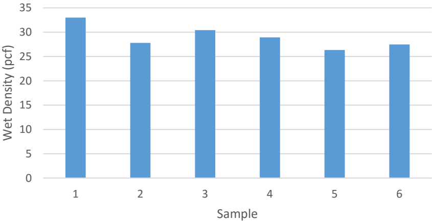
Figure 4-1: Wet density by sample for 0° skew test.
