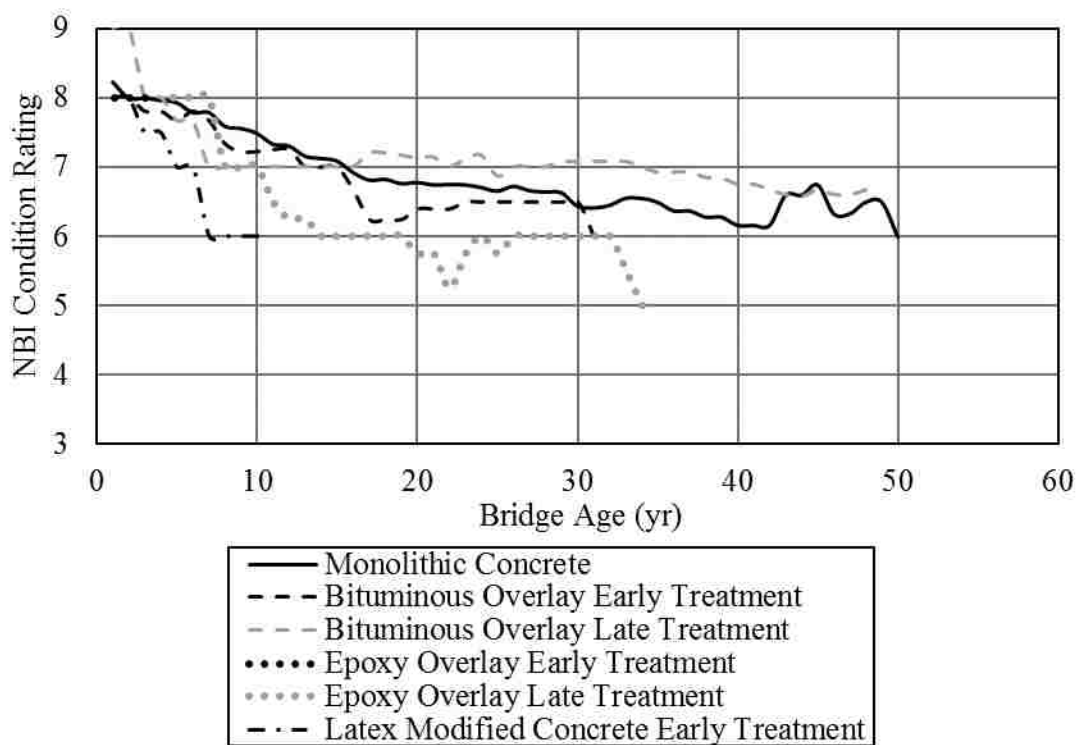
Figure 4-4: Average deterioration curves aligned by deck construction time for Region 4.
